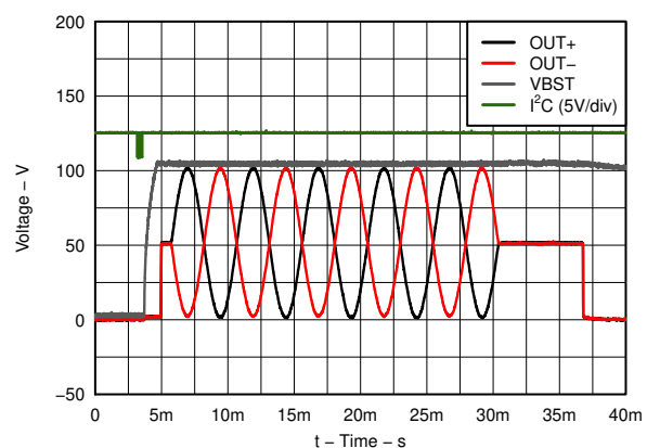
Figure 8-4. Typical Waveform
