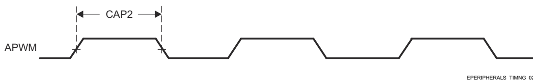
Figure 6-57. eCAP Output Timings
