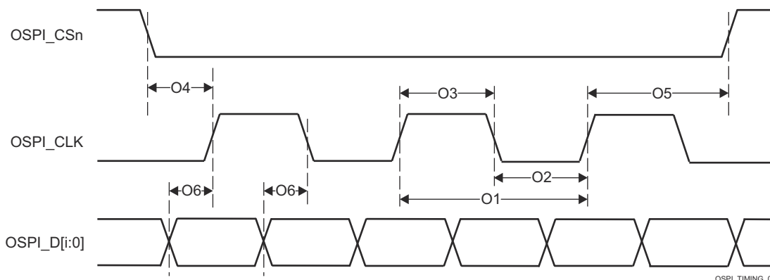
Figure 6-118. OSPI Switching Characteristics – Tap DDR, No Loopback
