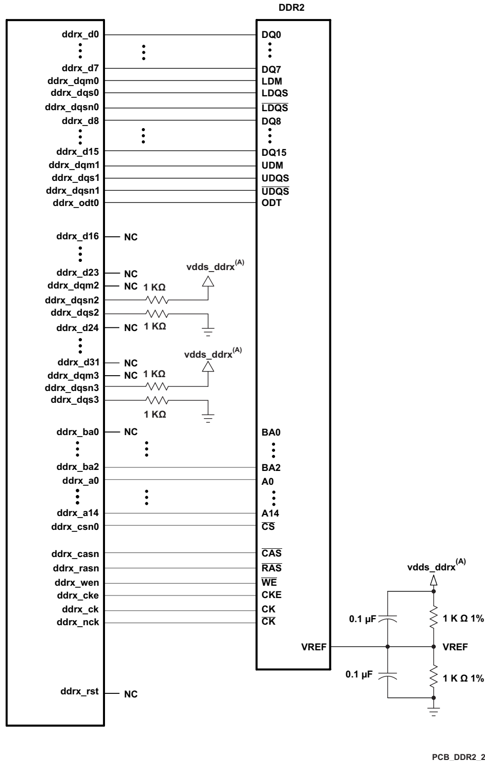
Figure 7-25. 16-Bit DDR2 High-Level Schematic
