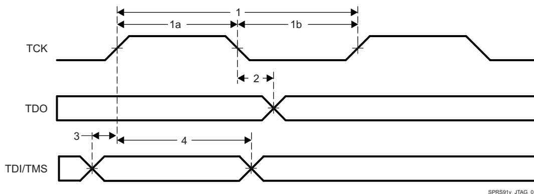
Figure 5-63. JTAG Timing
