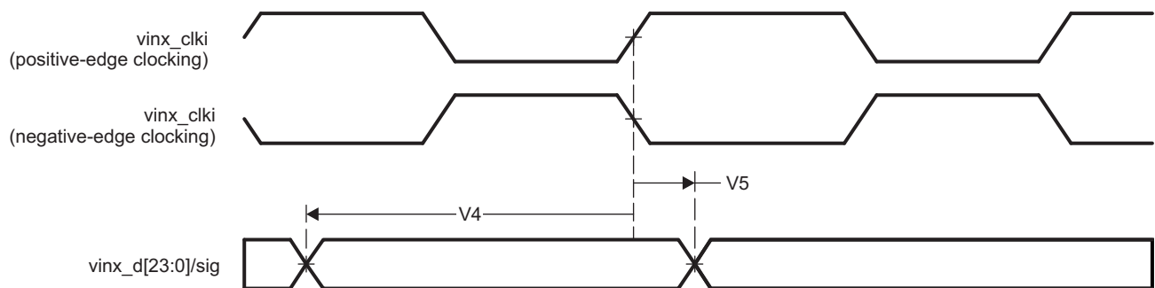
Figure 5-20. Video Input Ports Timings
