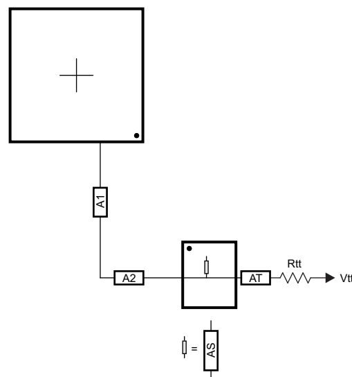
Figure 7-49. CK Routing for One DDR3 Device
