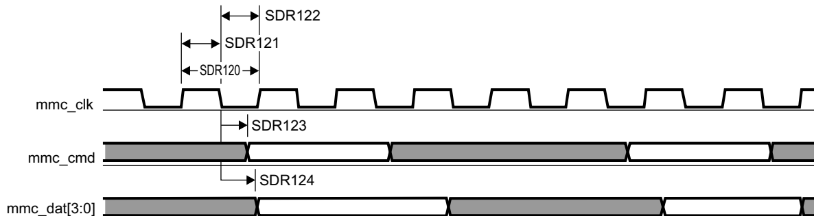
Figure 5-59. MMC/SD/SDIOj in - SDR12 - Transmitter Mode
