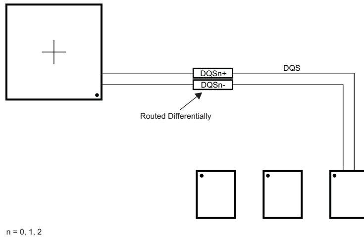
Figure 7-53. DQS Routing With Any Number of Allowed DDR3 Devices
