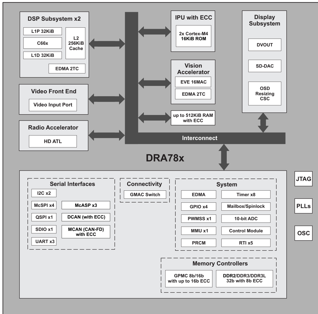
Figure 1-1. DRA78x Block Diagram
