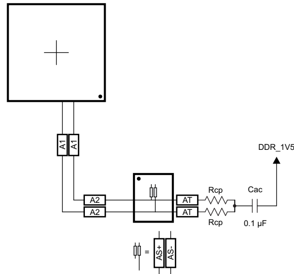
Figure 7-49. CK Routing for One DDR3 Device
