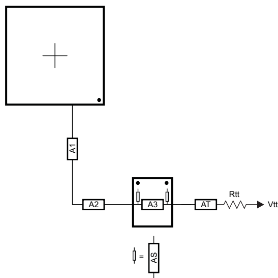
Figure 7-40. ADDR_CTRL Routing for Two Mirrored DDR3 Devices
