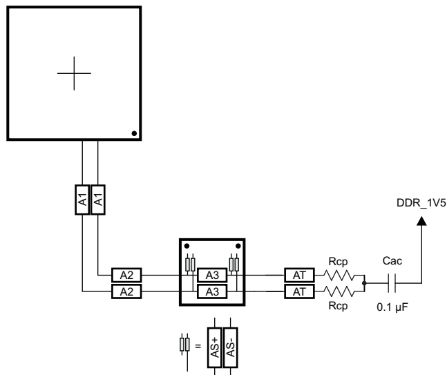
Figure 7-39. CK Routing for Two Mirrored DDR3 Devices
