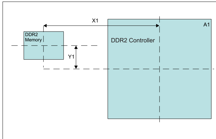
Figure 7-26. Device and DDR2 Device Placement
