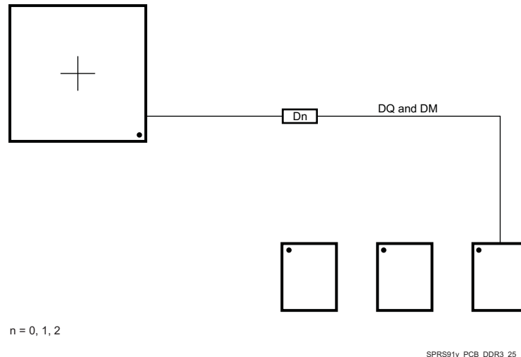
Figure 7-54. DQ/DM Routing With Any Number of Allowed DDR3 Devices
