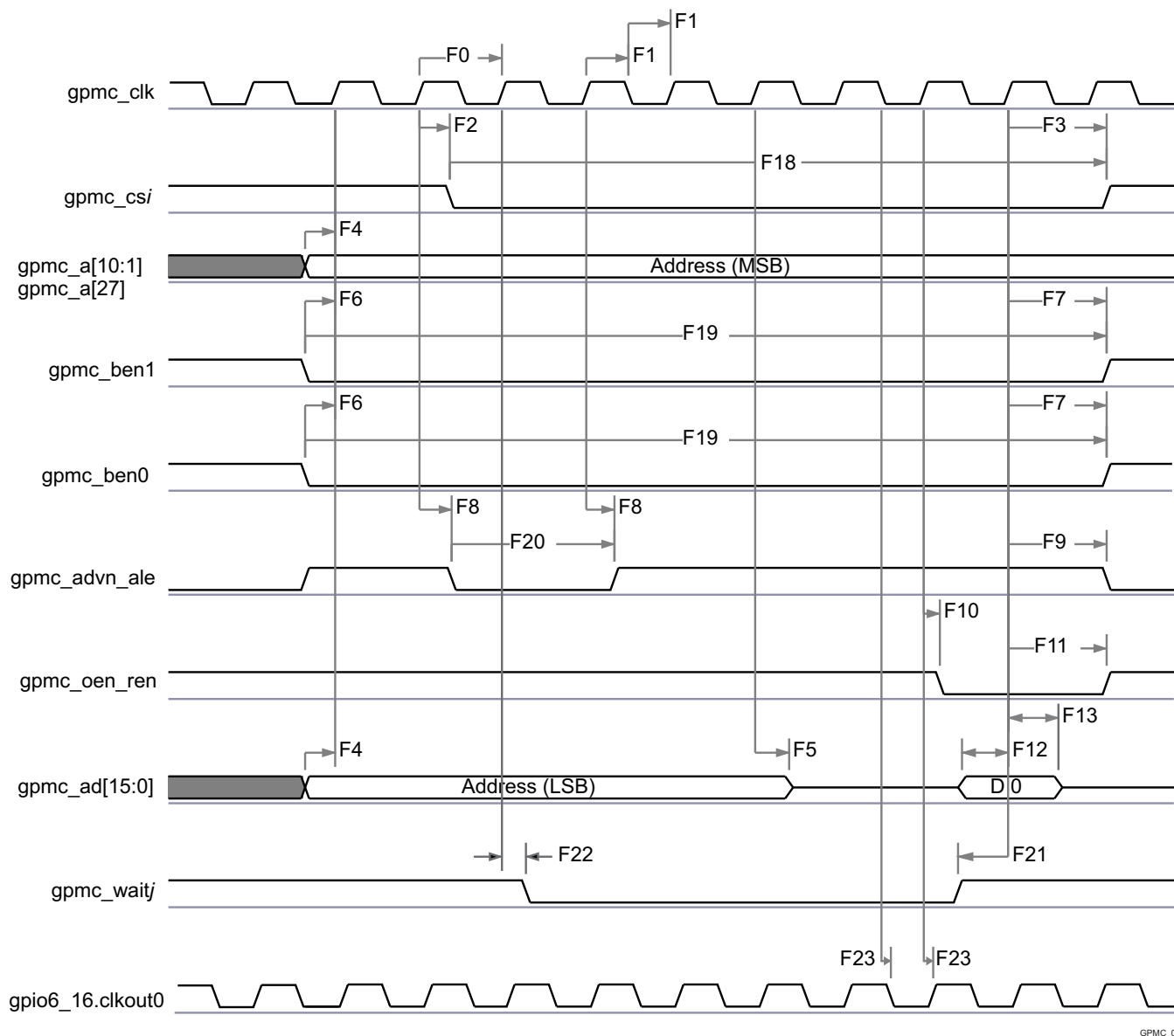
Figure 5-22. GPMC / Multiplexed 16bits NOR Flash - Synchronous Single Read - (GpmcFCLKDivider = 0) (1)(2)
