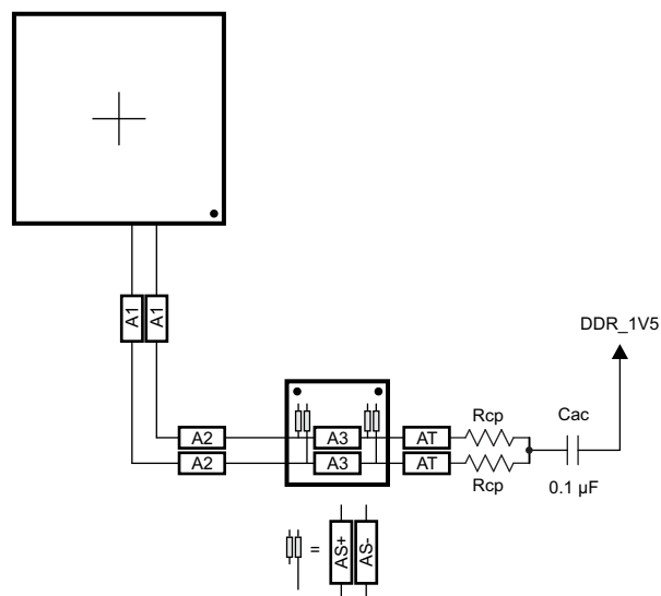
Figure 7-45. CK Routing for Two Mirrored DDR3 Devices
