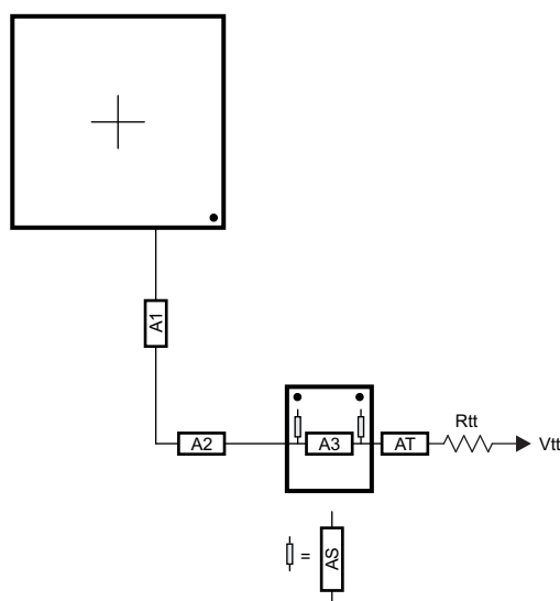
Figure 7-45. CK Routing for Two Mirrored DDR3 Devices
