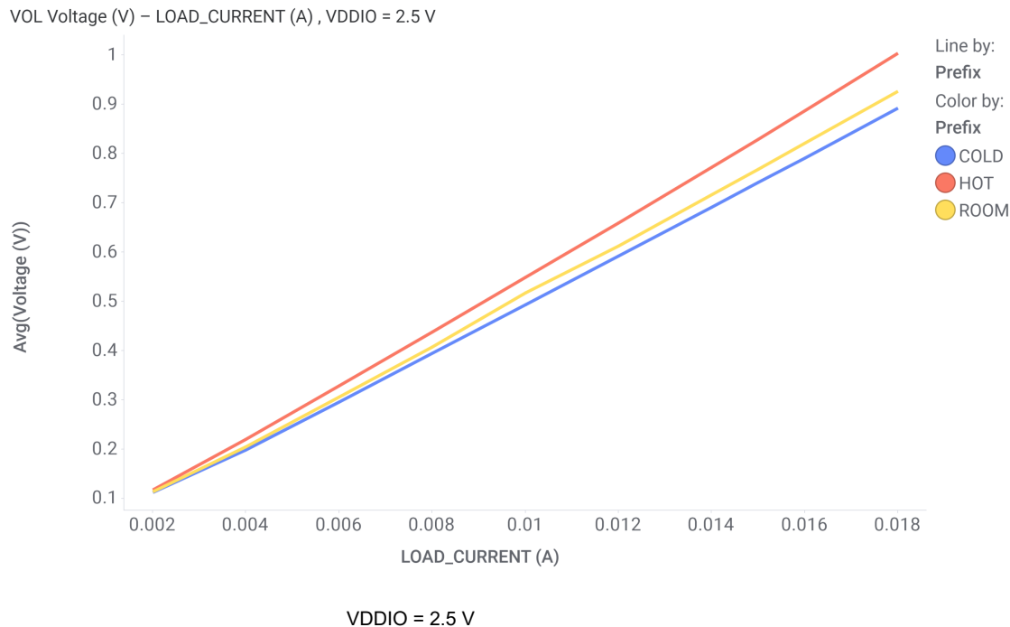
Figure 7-10. LED pins VOL (2.5 V)
