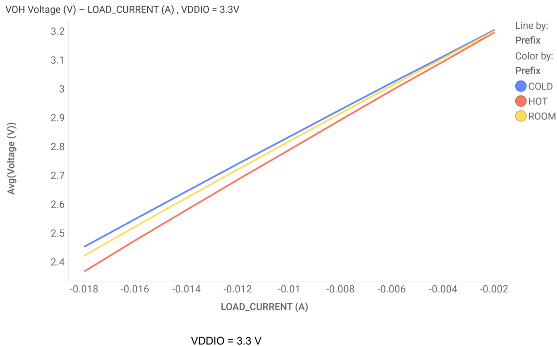
Figure 7-13. LED pins VOH (3.3 V)
