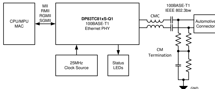
Simplified Schematic
