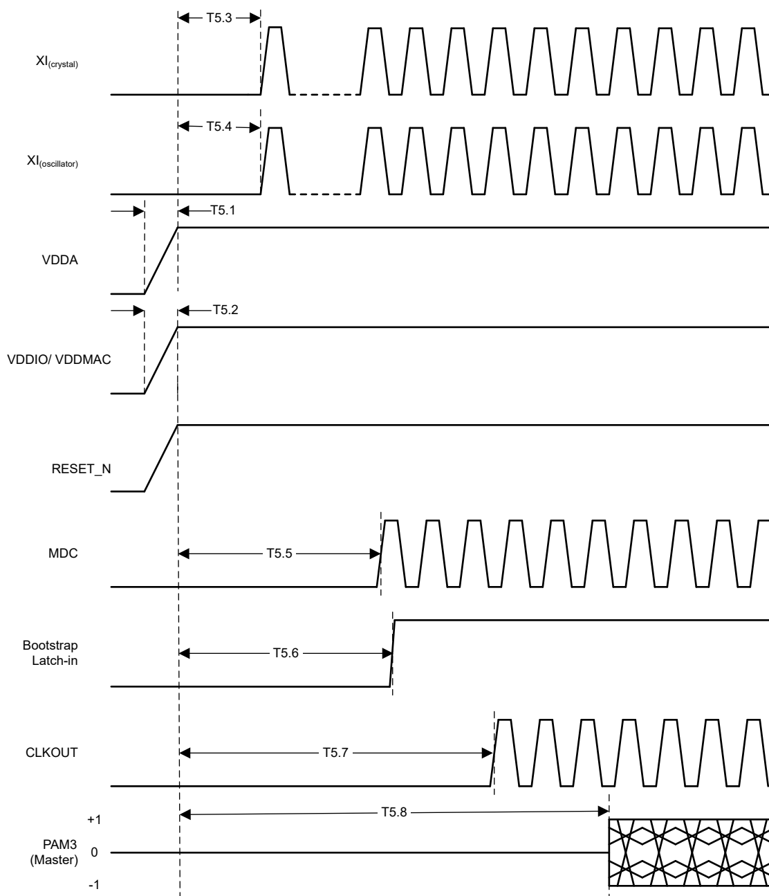
Figure 7-8. Power-Up Timing
