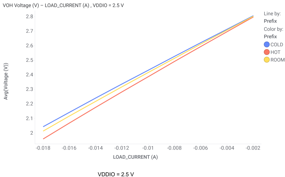
Figure 7-11. LED pins VOH (2.5 V)
