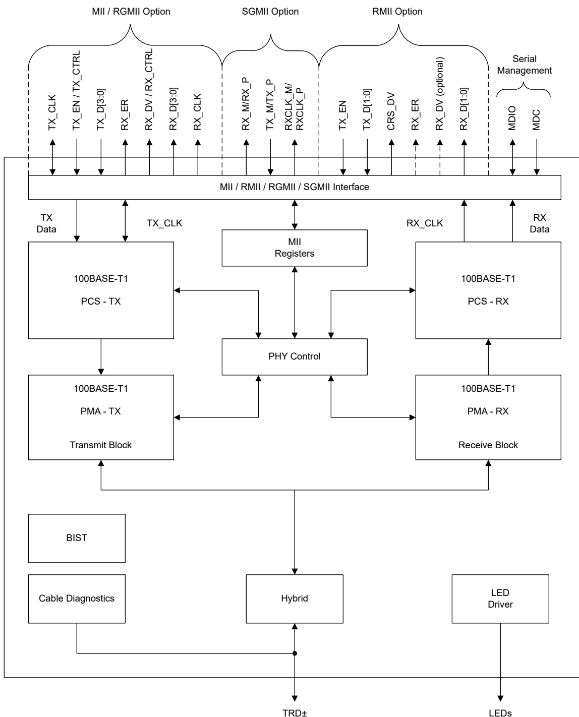
Figure 8-1. DP83TC814S-Q1
