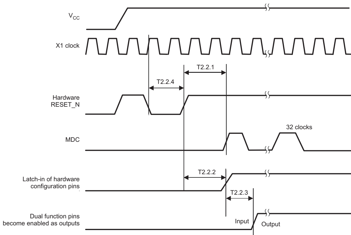
Figure 4-3. Reset Timing
