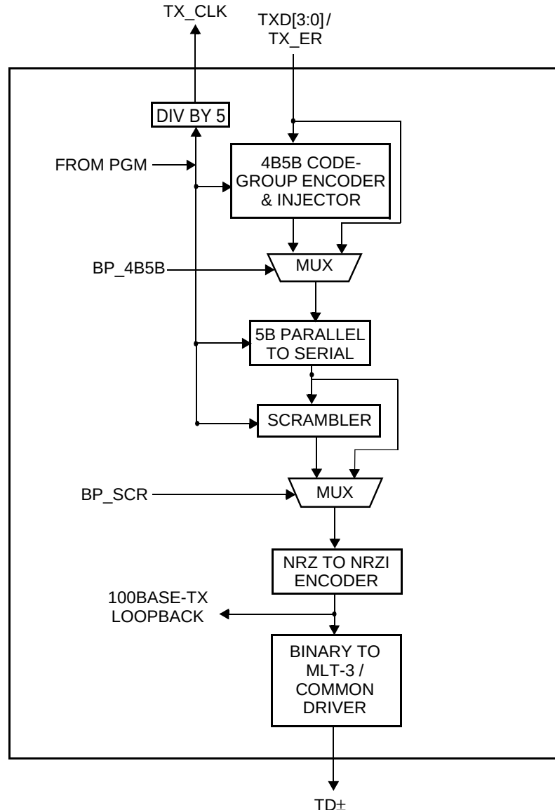
Figure 4. 100BASE-TX Transmit Block Diagram
