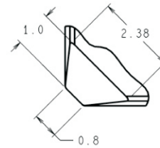
OPTIONAL PIN 1 CORNER
