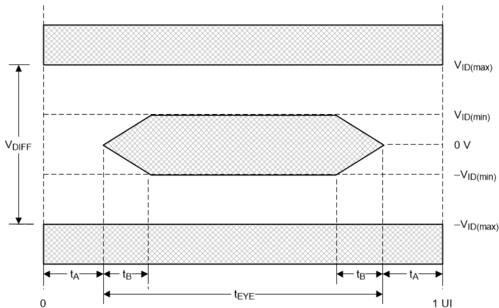
Figure 6-8. V-by-One Timing
