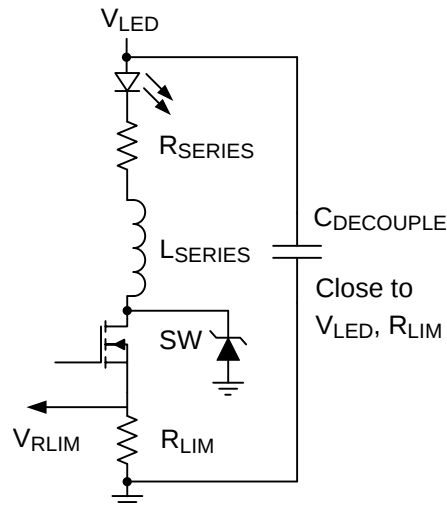
Figure 32. Parasitic Inductance ( L_{\text{Series}} ) and Resistance ( R_{\text{Series}} ) in Series with LED
