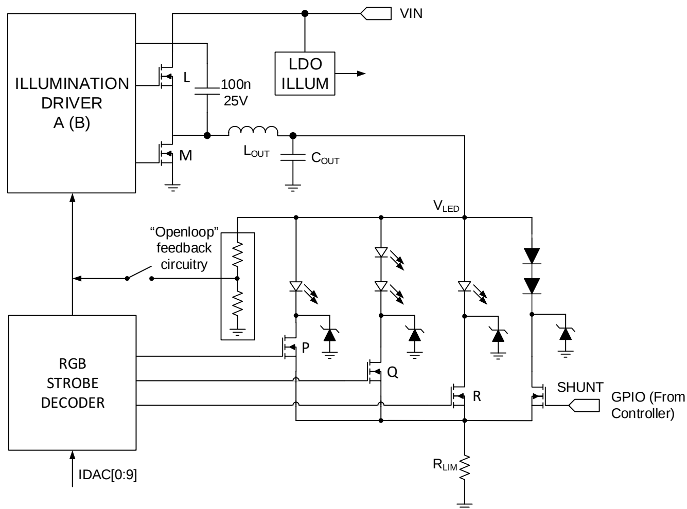
Figure 4. Illumination Control Loop
