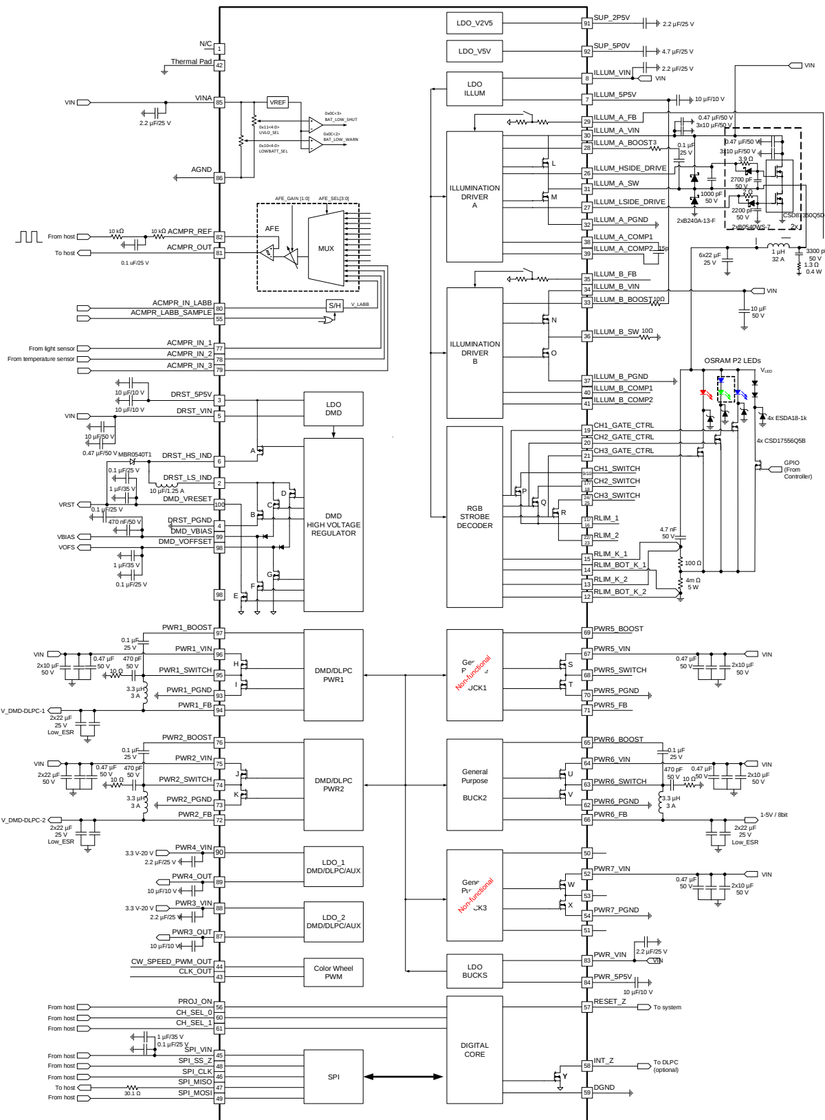
Figure 22. Typical Application: V_{IN} = 19.5\text{ V} , I_{OUT} = 32\text{ A} , LED, External MOSFETs
