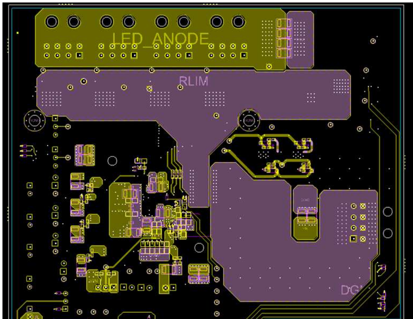
Figure 28. Current Return Path
