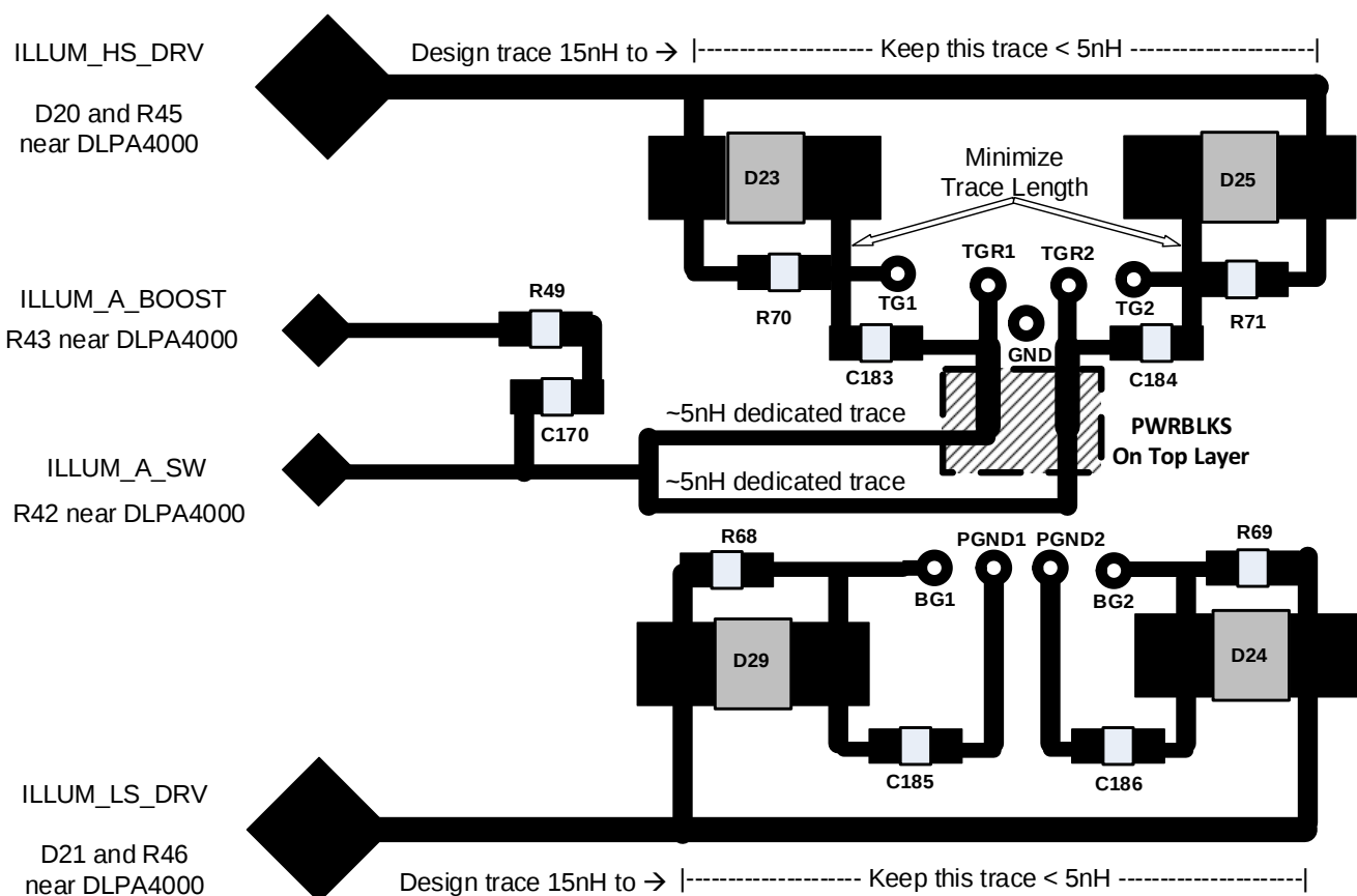
Figure 26. DLPA4000 Illumination Bottom Layout
