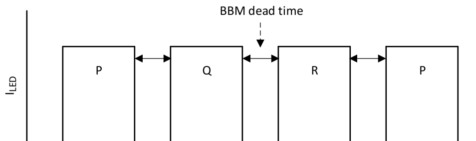
Figure 6-7. BBM Timing
