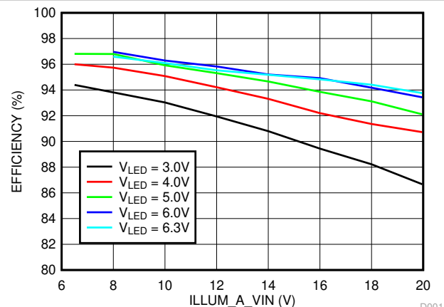
Figure 6-11. Illumination Driver Plus Power FETs Efficiency vs V_{ILLUM\_A\_IN} ( I_{OUT} = 16A )
