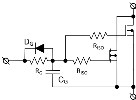
Figure 6-5. Using R_{SO} to Prevent Gate Oscillations When Using Power FETs in Parallel
