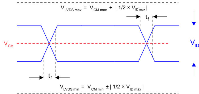
Figure 6-2. LVDS Waveform Requirements
