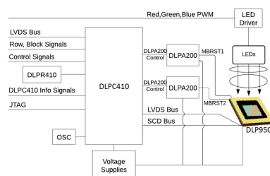
Simplified Schematic
