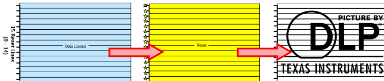
Figure 8-9. Global Mode
