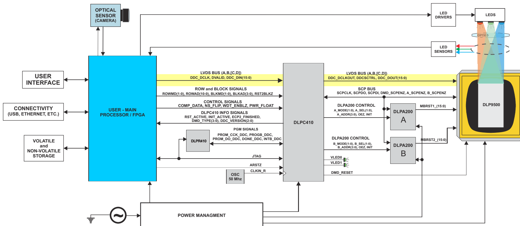
Figure 9-1. DLPC410 and DLP9500 Embedded Example Block Diagram
