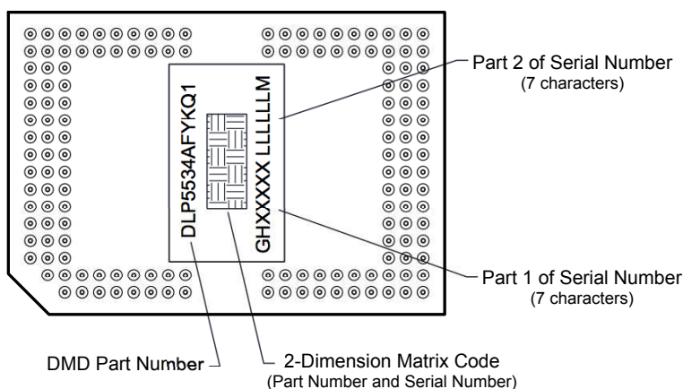
Figure 23. DMD Marking
