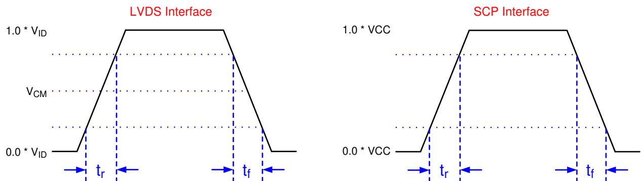
Figure 5-2. SCP Timing Parameters
