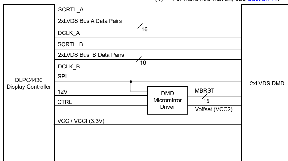
DLP550JE Simplified Application
