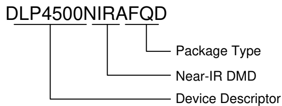
Figure 12-1. Device Nomenclature
