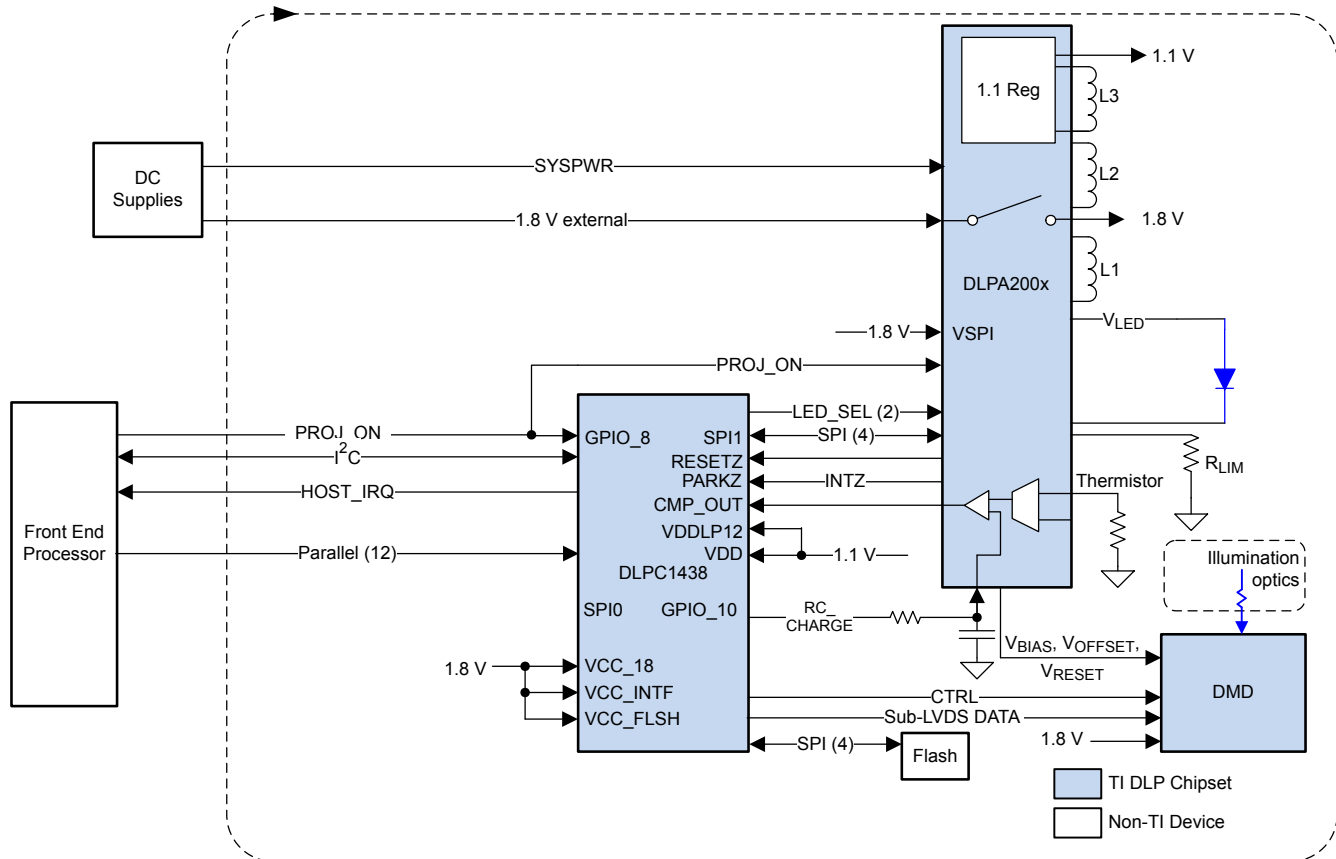
Figure 8-2. Without FPGA
