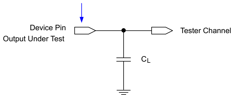
Figure 6-14. Test Load Circuit for Output Propagation Measurement
