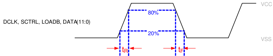
Figure 6-4. Rise and Fall Timing Parameters 1
