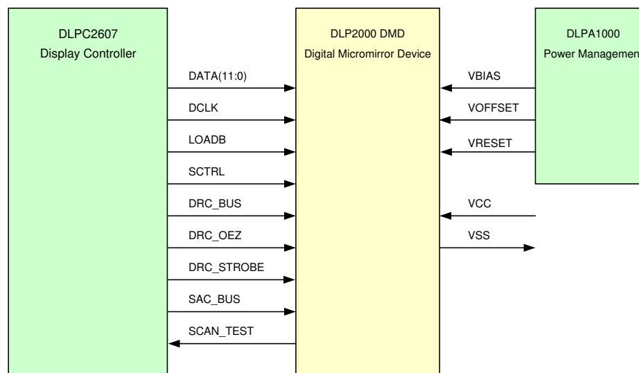
Simplified Application
