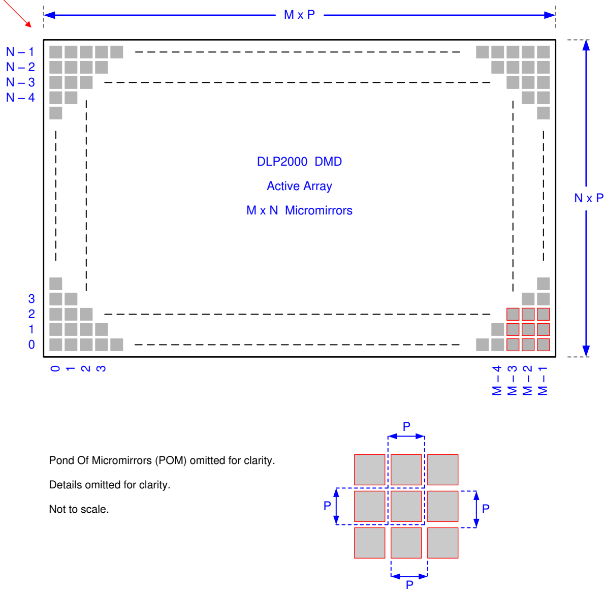
Figure 6-8. Micromirror Array Physical Characteristics
