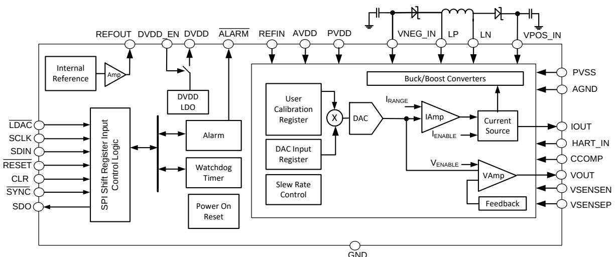
DAC8771 Block Diagram
