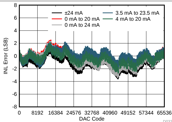
Figure 36. IOUT INL vs Code (DC/DC Enabled)
