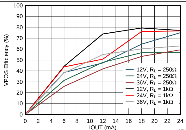
Figure 79. IOU VPOS Efficiency
