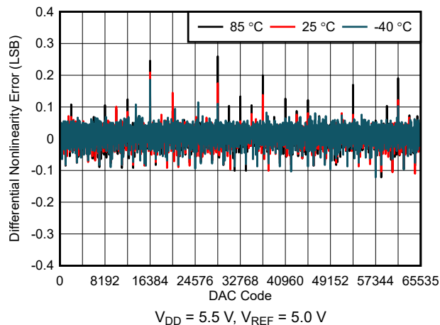
Figure 6-6. Differential Linearity Error vs Digital Input Code
