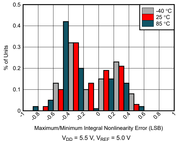
Figure 6-4. Integral Linearity Error Histogram
