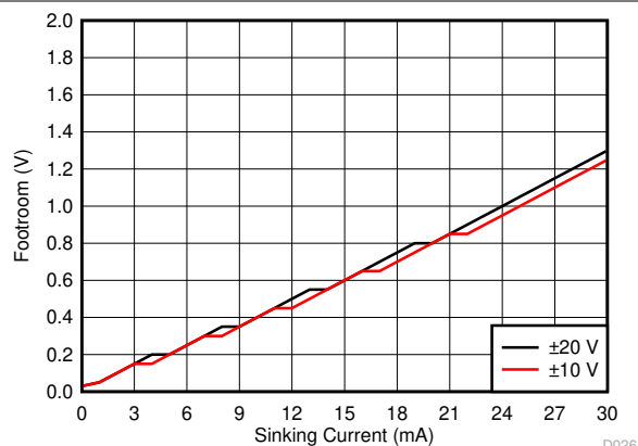
Figure 5-29. V_{SS} Footroom vs Sinking Current
