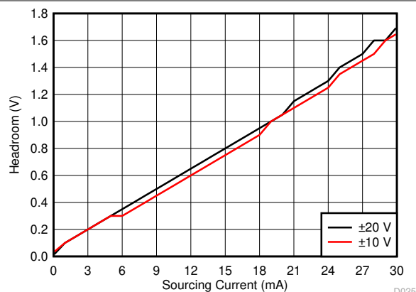
Figure 5-28. V_{CC} Headroom vs Sourcing Current
