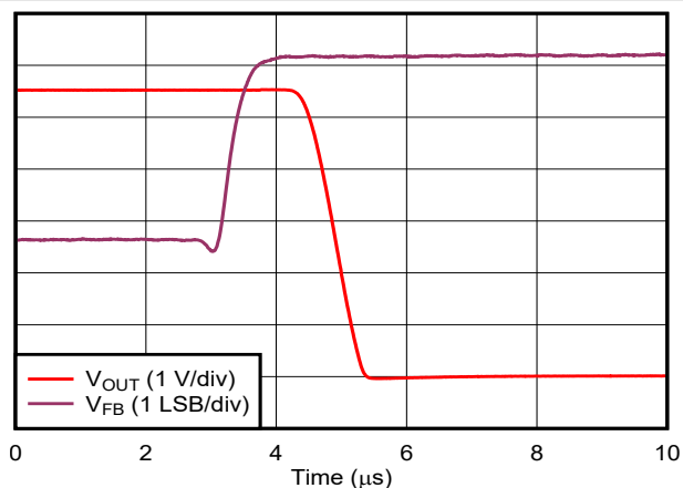
Figure 6-58. Comparator Response Time: High-to-Low Transition
