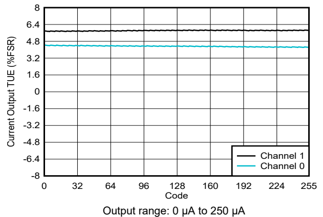
Figure 6-41. Current Output TUE vs Digital Input Code
