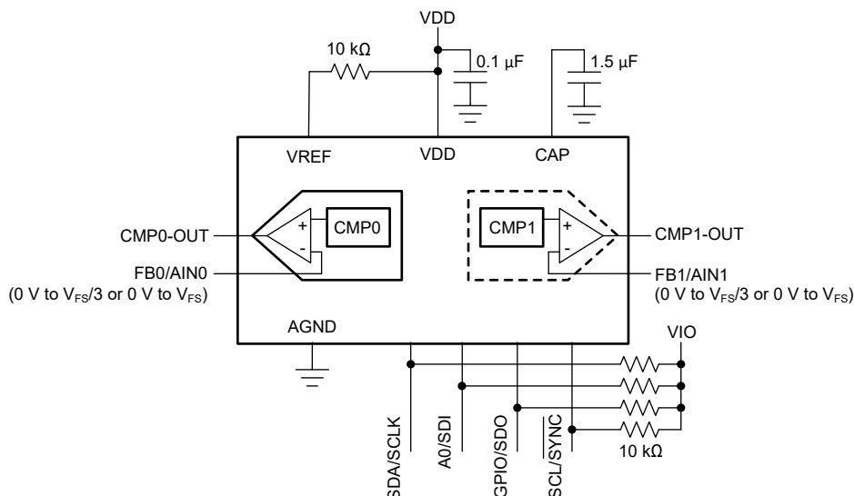
Figure 7-3. Comparator Interface
