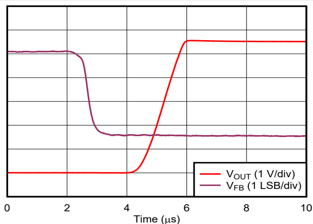
Figure 6-57. Comparator Response Time: Low-to-High Transition
