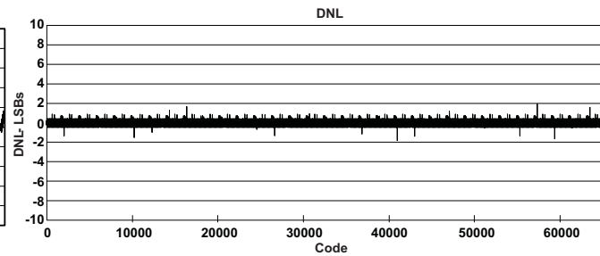
Figure 2. Differential Nonlinearity
