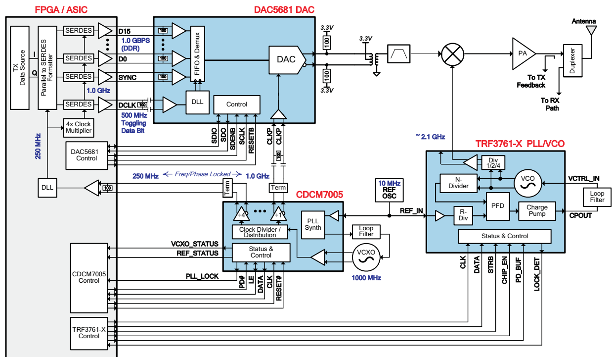
Figure 24. Example Direct Conversion System Diagram
