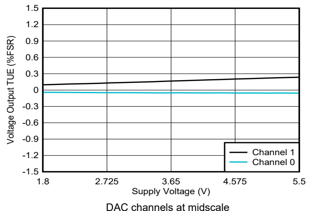
Figure 6-15. Voltage Output TUE vs Supply Voltage
