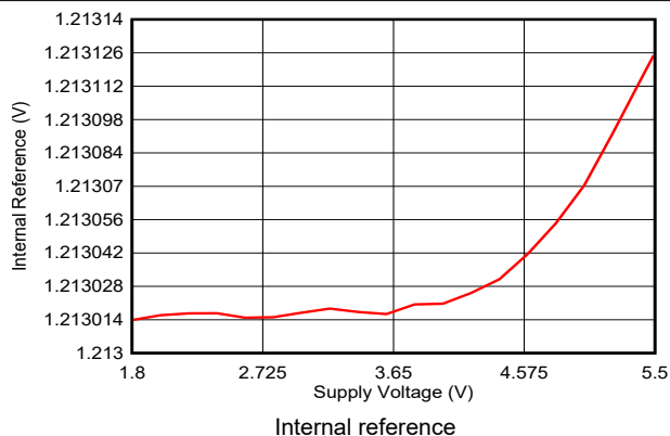
Figure 6-63. Internal Reference vs Supply Voltage
