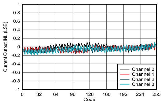
Figure 6-31. Current Output INL vs Digital Input Code
