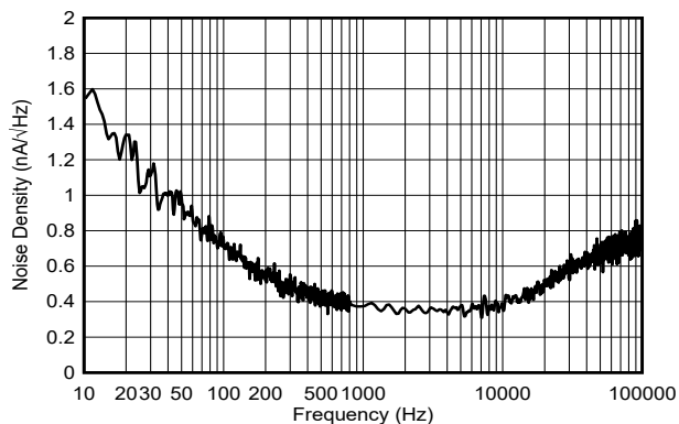
Figure 6-56. Current Output Noise Density
