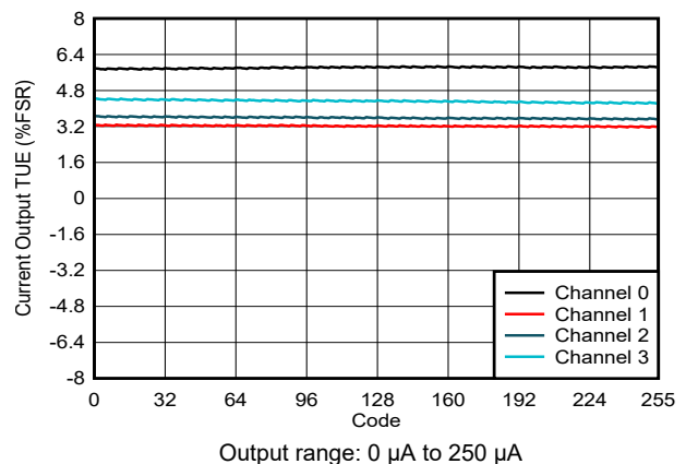
Figure 6-42. Current Output TUE vs Digital Input Code
