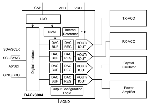
DACx3004 for Biasing in Land Mobile Radio
