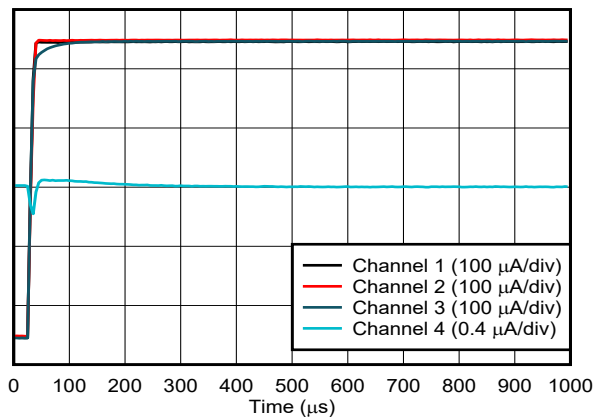
Figure 6-51. Current Output Power-On Glitch
