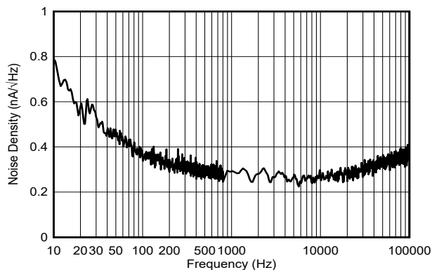
Figure 6-55. Current Output Noise Density
