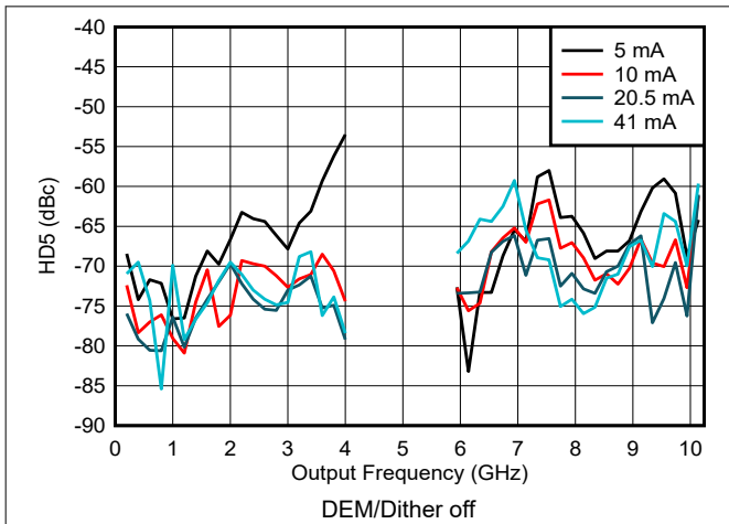
Figure 6-179. HD5 vs Frequency and Output Current in DES2X Modes
