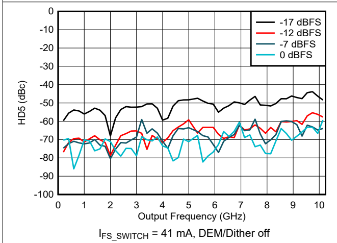
Figure 6-183. HD5 vs Frequency and Digital Amplitude in NRZ/RF Modes
