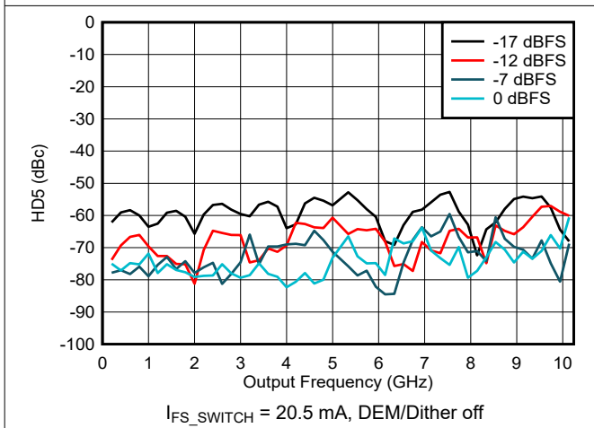
Figure 6-181. HD5 vs Frequency and Digital Amplitude in NRZ/RF Modes
