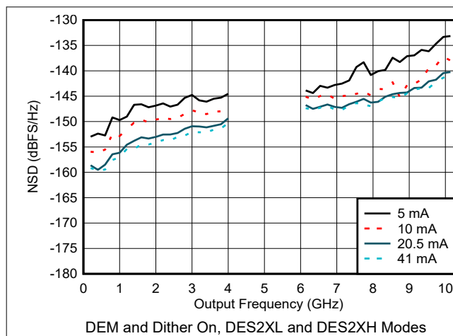
Figure 6-64. NSD vs Output Frequency and Output Current
