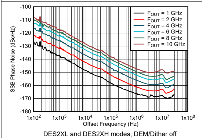
Figure 6-203. Phase Noise vs Offset Frequency and Output Frequency
