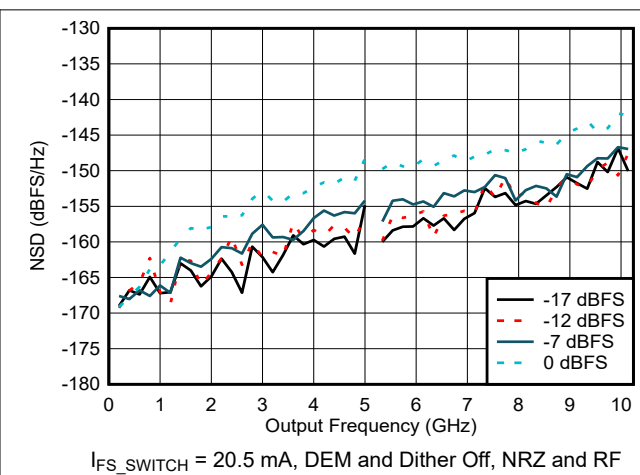
Figure 6-65. NSD vs Output Frequency and Digital Amplitude
