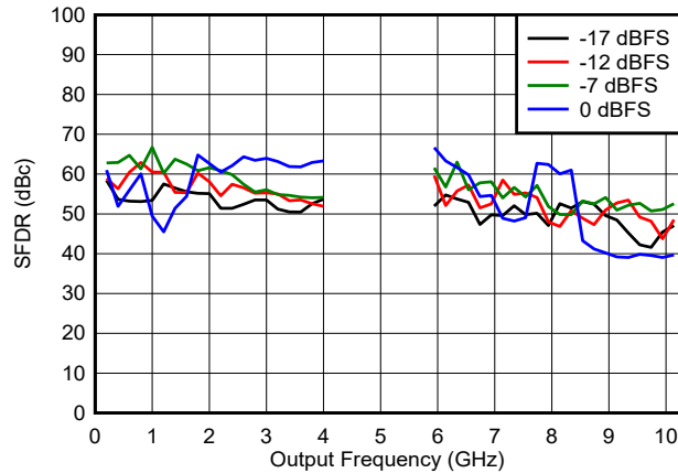
Figure 6-122. SFDR vs Frequency and Digital Amplitude in DES2X Modes
