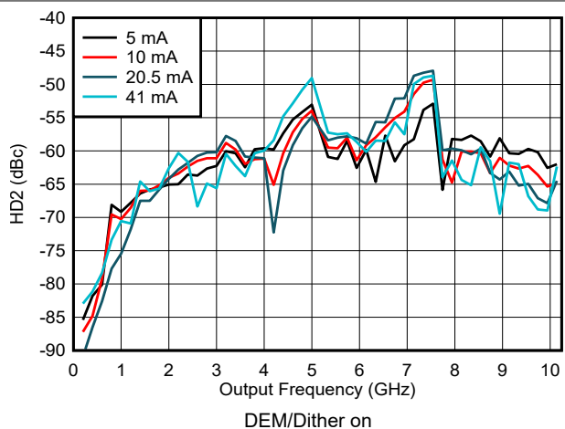
Figure 6-157. HD2 vs Frequency and Output Current in NRZ/RF Modes
