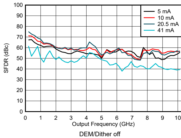
Figure 6-112. SFDR vs Frequency and Output Current in NRZ/RF Modes
