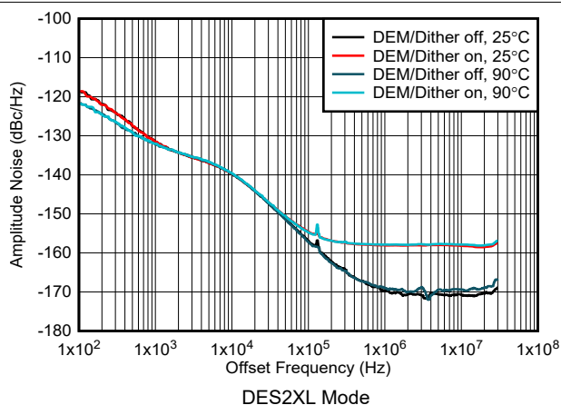
Figure 6-225. Amplitude Noise vs Offset Frequency and Temperature at 1GHz
