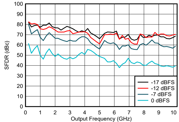
Figure 6-117. SFDR vs Frequency and Digital Amplitude in NRZ/RF Modes
