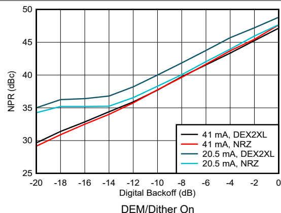
Figure 6-211. Noise Power Ratio vs Digital Backoff: 1 st Nyquist Zone
