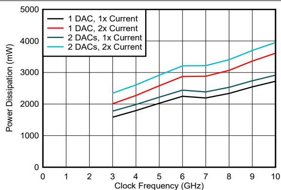
Figure 6-91. Power Dissipation vs Clock Frequency and DAC Mode
