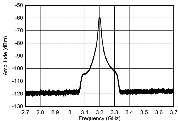
Figure 8-18. NLFM Chirp Output Spectra across 1GHz
