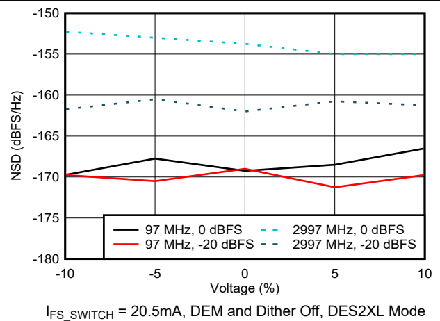
Figure 6-87. NSD vs Supply Voltage
