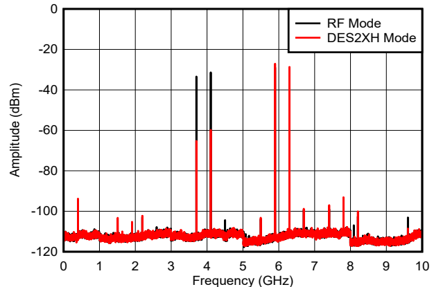
Figure 6-52. Dual Tone, f_{\text{OUT}} = 6097\text{MHz} , 0dBFS
