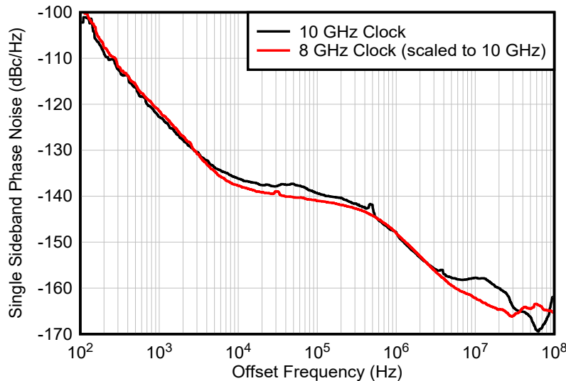
Figure 8-12. 8GHz and 10GHz Clock Phase Noise
