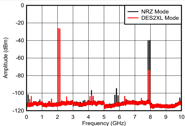
Figure 6-46. Dual Tone, f_{\text{OUT}} = 2097\text{MHz} , 0dBFS
