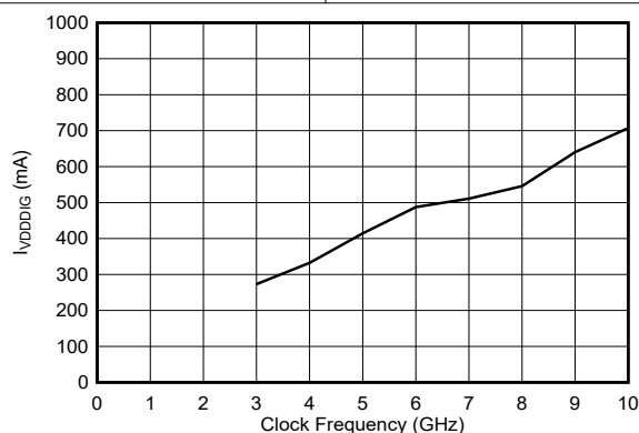
Figure 6-102. VDDDIG Current vs Clock Frequency and Digital Mode
