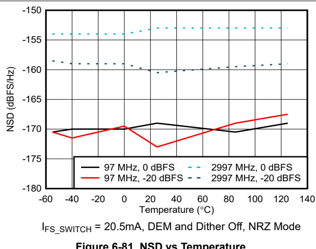
Figure 6-81. NSD vs Temperature
