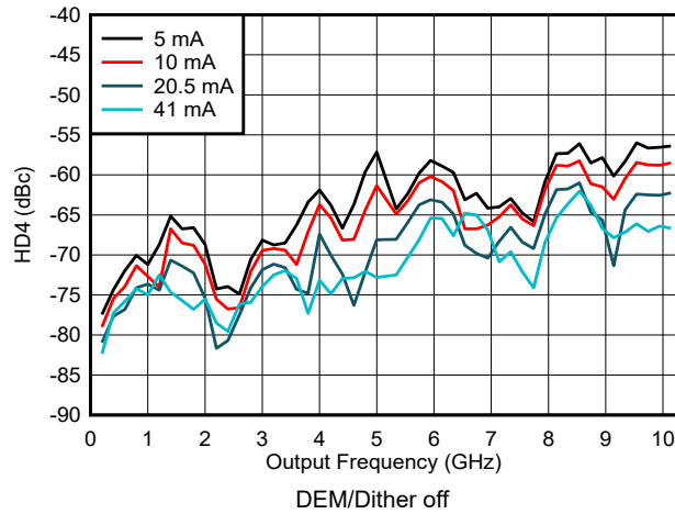
Figure 6-188. HD4 vs Frequency and Output Current in NRZ/RF Modes
