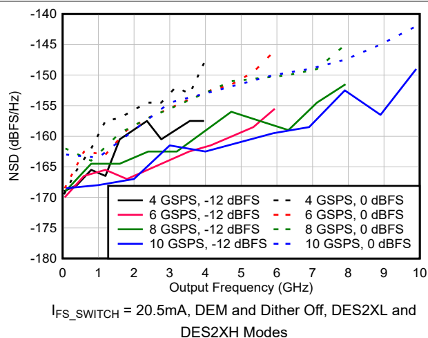
Figure 6-79. NSD vs Output Frequency and Sample Rate
