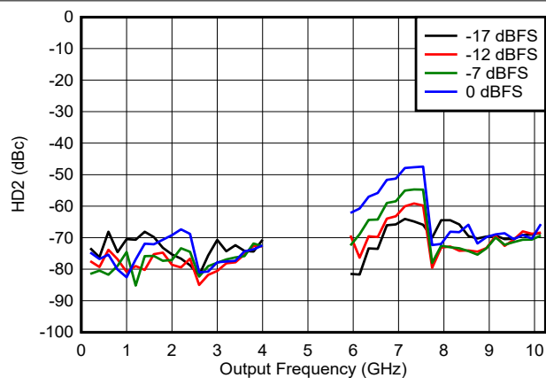
Figure 6-165. HD2 vs Frequency and Digital Amplitude in DES2X Modes
