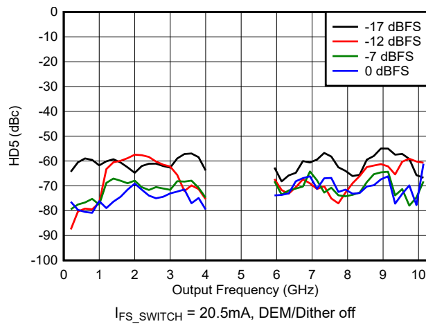
Figure 6-200. HD5 vs Frequency and Digital Amplitude in DES2X Modes
