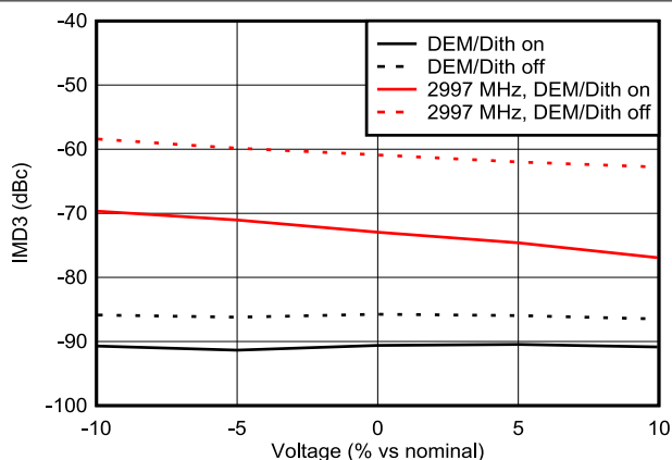
Figure 6-153. IMD3 vs Voltage in DES2XL Mode
