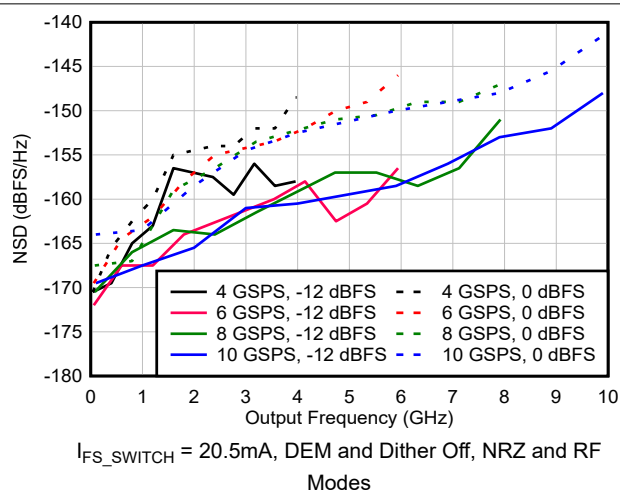
Figure 6-77. NSD vs Output Frequency and Sample Rate
