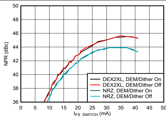
Figure 6-215. Noise Power Ratio vs Output Current: 2 nd Nyquist Zone
