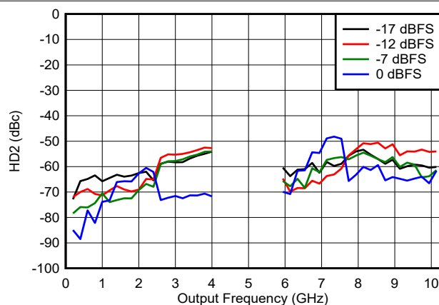
Figure 6-164. HD2 vs Frequency and Digital Amplitude in DES2X Modes
