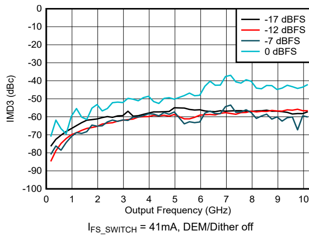
Figure 6-134. IMD3 vs Frequency and Digital Amplitude in NRZ/RF Modes
