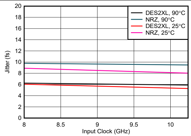
Figure 6-221. Jitter vs Input Clock
