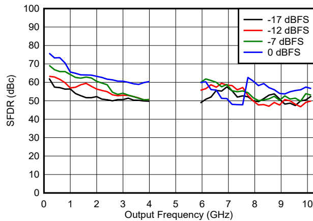
Figure 6-120. SFDR vs Frequency and Digital Amplitude in DES2X Modes
