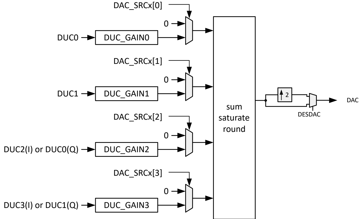
Figure 7-47. Channel Bonder Block Diagram
