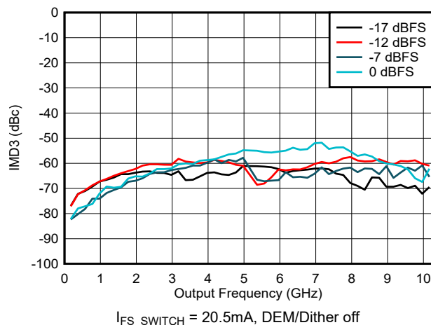
Figure 6-132. IMD3 vs Frequency and Digital Amplitude in NRZ/RF Modes
