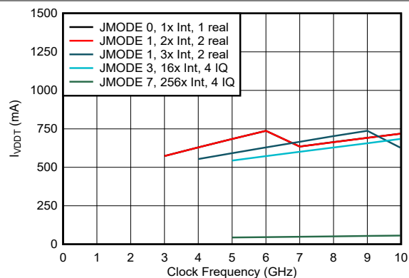
Figure 6-101. VDDT Current vs Clock Frequency and Mode
