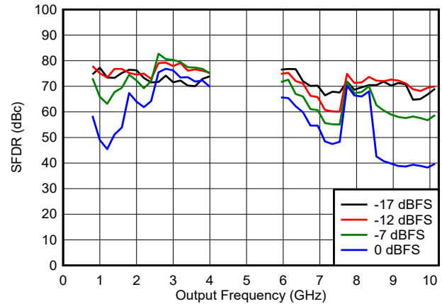
Figure 6-123. SFDR vs Frequency and Digital Amplitude in DES2X Modes
