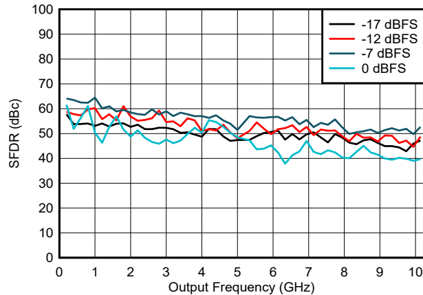
Figure 6-116. SFDR vs Frequency and Digital Amplitude in NRZ/RF Modes
