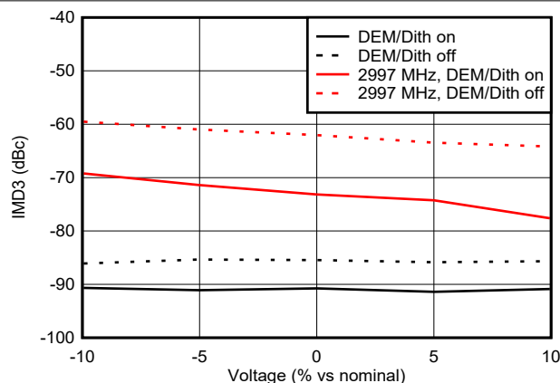
Figure 6-152. IMD3 vs Voltage in NRZ Mode
