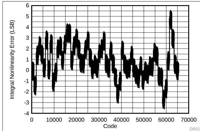
Figure 1. Integral Nonlinearity
