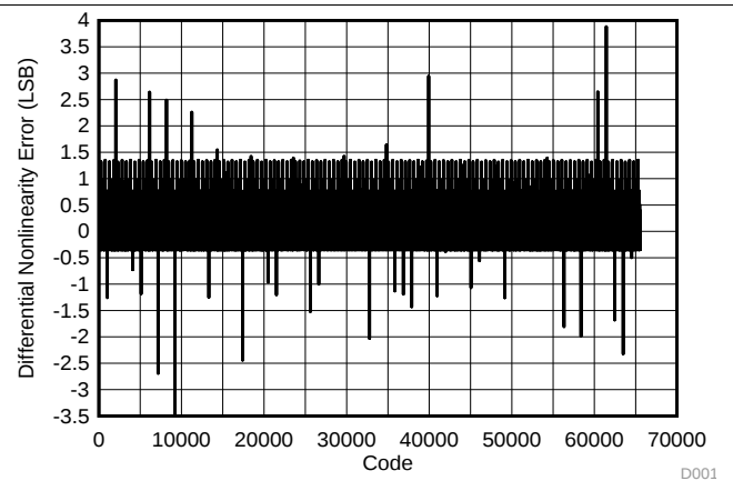
Figure 2. Differential Nonlinearity
