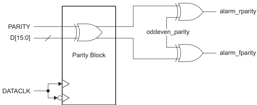
Figure 6-29. DAC3482 Word-by-Word Parity Check
