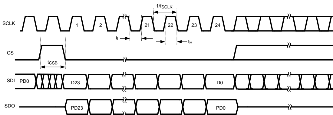
Figure 1. DAC161S055 Input/Output Waveforms
