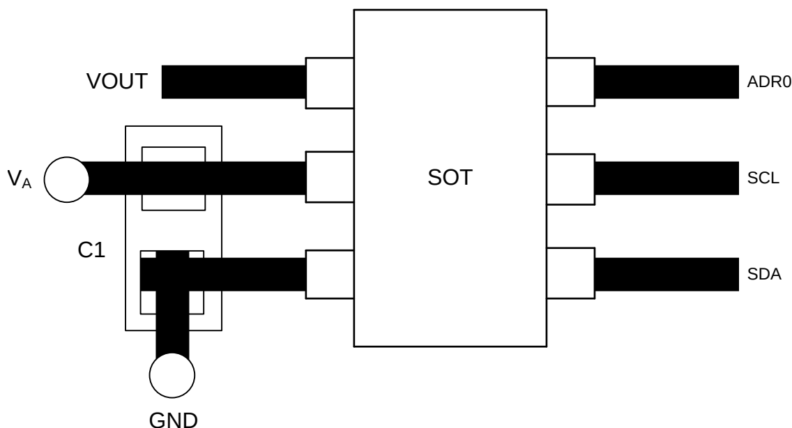
Figure 36. Typical Layout
