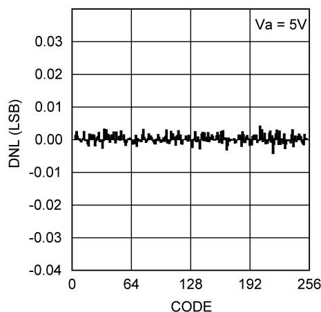
Figure 5. DNL
