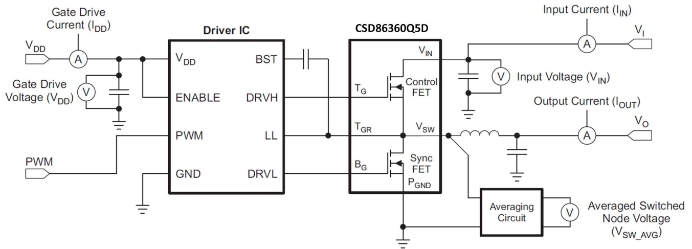
Figure 33. Typical Application
