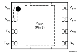
Figure 1. Top View
