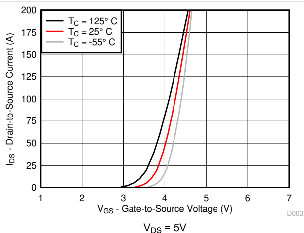
Figure 4-3. Transfer Characteristics
