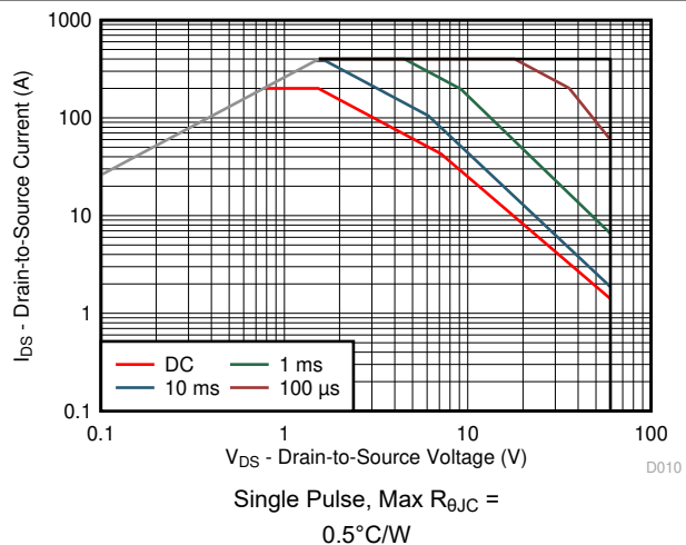
Figure 3-10. Maximum Safe Operating Area
