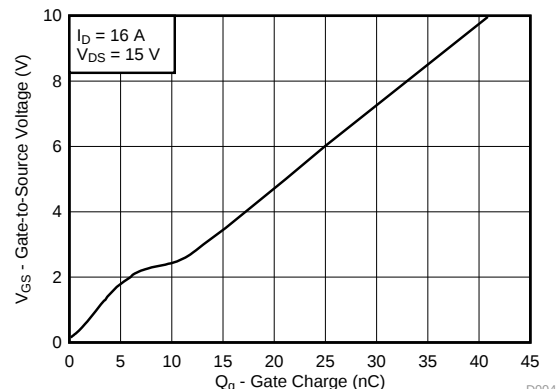
Gate Charge
