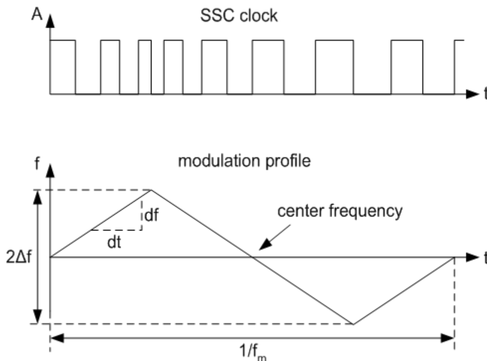
Figure 8-2. Modulation Frequency ( f_m ) and Modulation Amount
