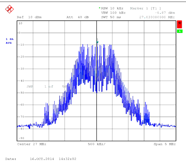
Figure 8-10. Output Spectrum With SSC On, 2% Center
