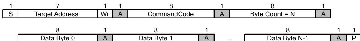
Figure 7-6. Block Write Protocol
