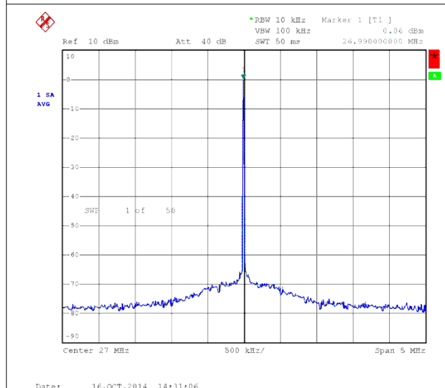
Figure 8-9. Output Spectrum With SSC Off
