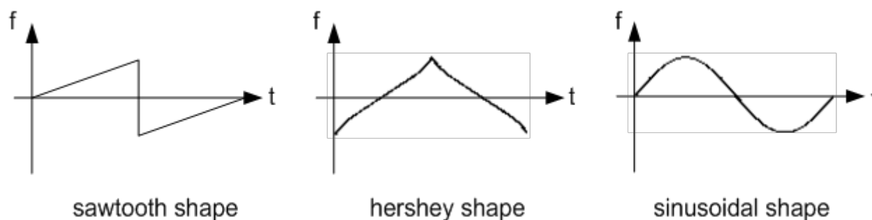
Figure 8-3. Spread Spectrum Modulation Shapes
