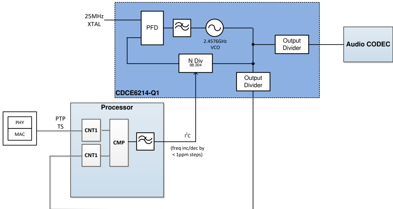
Figure 11-2. eAVB System Block Diagram Using CDCE6214Q1TM
