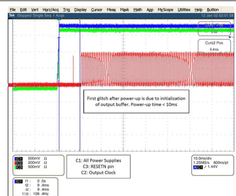
Figure 5-5. All Power Supply = 1.8 V, VDD Ramp Time = 1 ms
