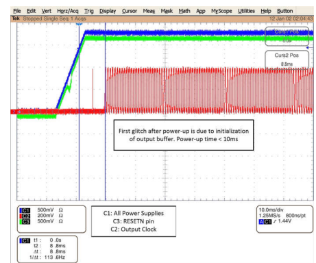
Figure 5-7. All Power Supply = 1.8 V, VDD Ramp Time = 10 ms
