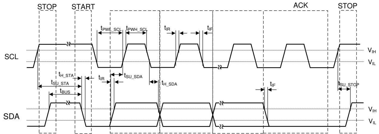
Figure 6-7. I²C Timing
