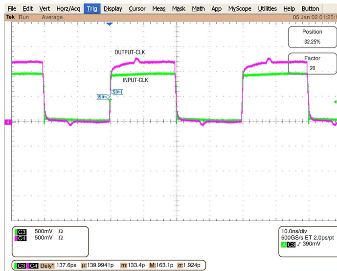
Figure 7-2. Input/Output Alignment in External Zero Delay Mode for LVCMOS Output
