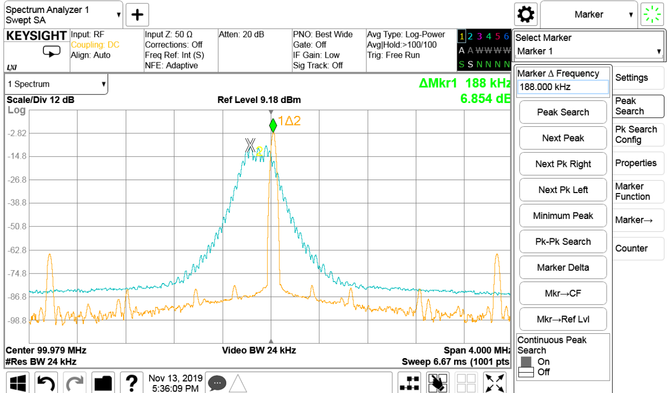
Figure 7-4. 100 MHz With -0.25\% Down Spread With and Without Trace
