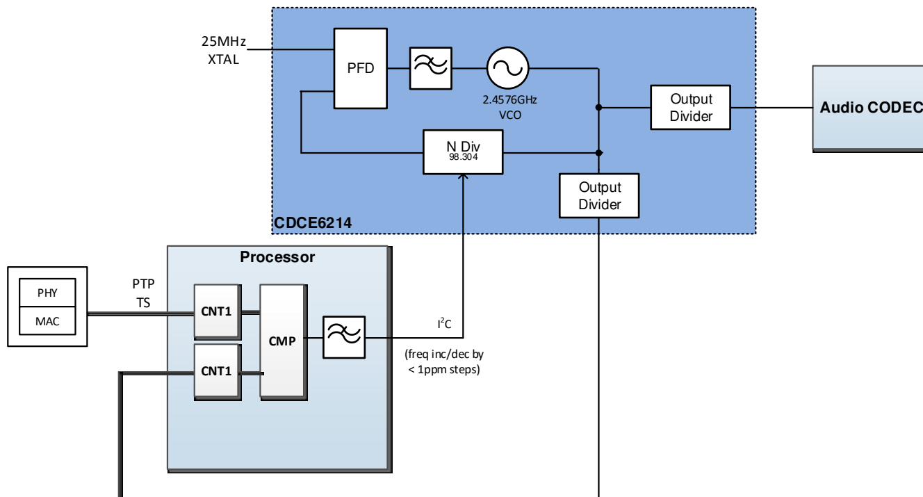
Figure 8-2. eAVB System Block Diagram Using CDCE6214
