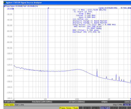
Reference: Crystal Closed-Loop Phase 24.576-MHz LVCMOS Input 25 MHz Noise from 2.4576-GHz VCO
