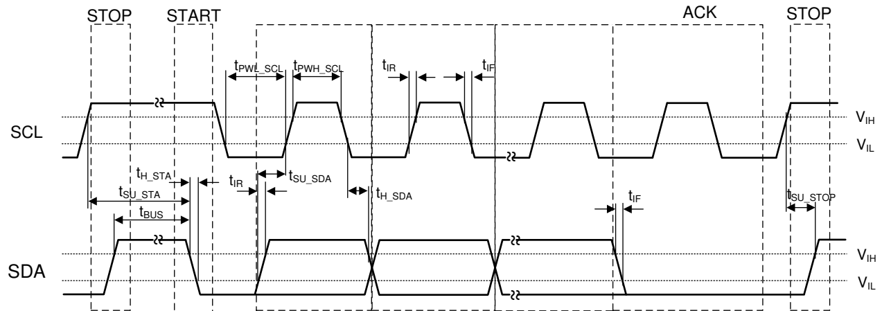
Figure 6-7. I 2 C Timing
