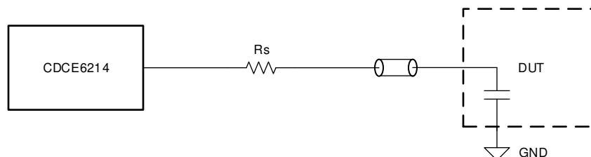
Figure 6-11. LVCMOS Output
