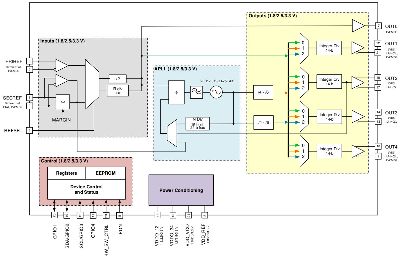
Figure 7-1. CDCE6214 Clock Generator With Two Inputs, One Fractional-N PLL, and Four Outputs
