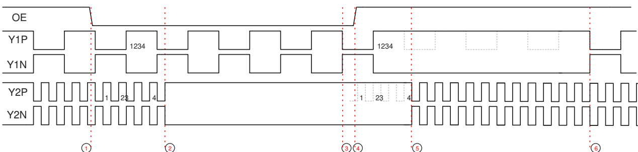
Figure 7-10. Individual Output Enable and Disable
