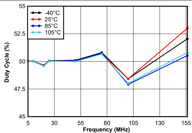
Figure 6-12. Duty Cycle vs Frequency and Temperature at 1.8V Supply, No Capacitive Load, Normal Mode Device
