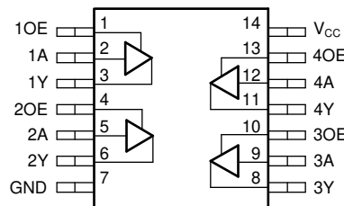
Functional pinout
