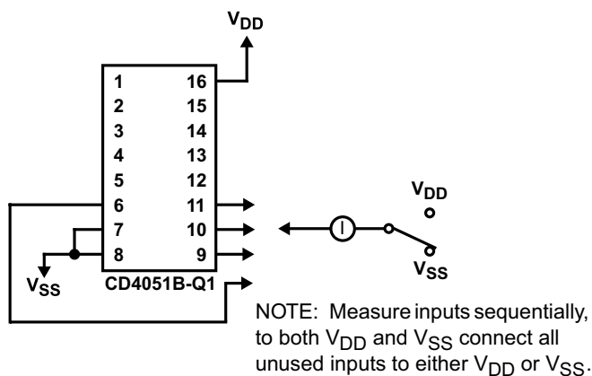
Figure 6-12. Input Current
