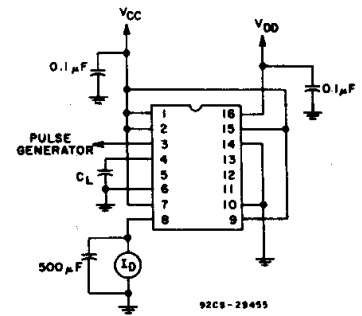
Fig. 16 - Dynamic power dissipation test circuit.
