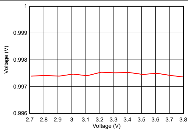
Figure 7-32. ADC Accuracy vs Supply Voltage ( V_{in}=1V , Internal Reference, 200ksps)
