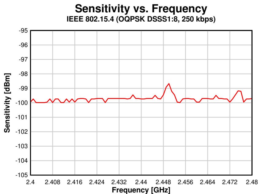
Figure 8-12. Sensitivity vs. Frequency IEEE 802.15.4 (OQPSK DSSS1:8, 250 kbps)
