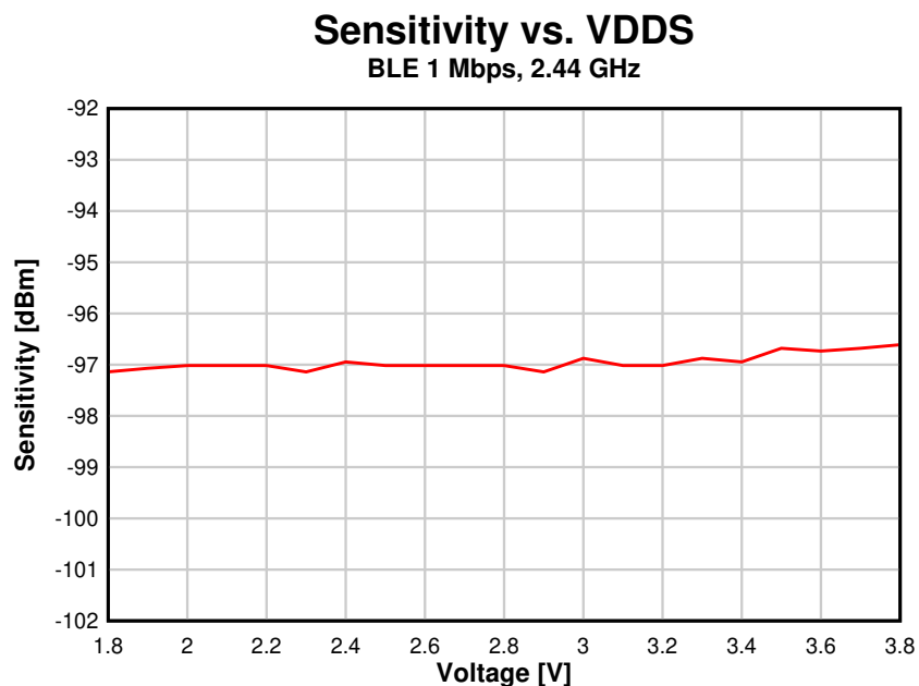
Figure 8-15. Sensitivity vs. Supply Voltage (VDDS) (BLE 1 Mbps, 2.44 GHz)
