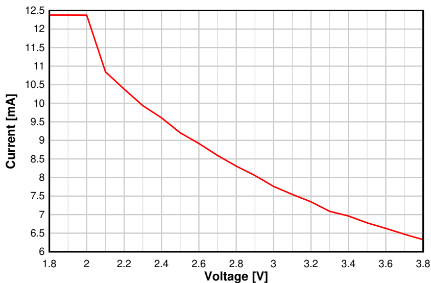
Figure 8-10. TX Current vs. Supply Voltage (VDD5) (BLE 1 Mbps, 2.44 GHz)
