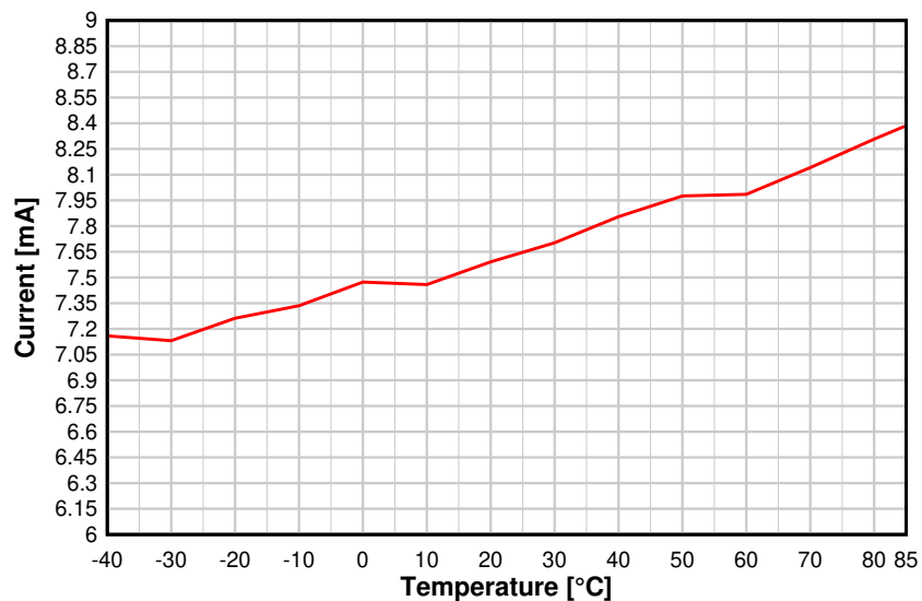
Figure 8-9. TX Current vs. Temperature (BLE 1 Mbps, 2.44 GHz)
