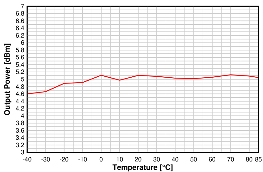
Figure 8-19. Output Power vs. Temperature (BLE 1 Mbps, 2.44 GHz, +5 dBm)
