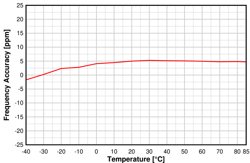
Figure 8-24. Compensated Frequency Accuracy vs. Temperature (2.44 GHz)
