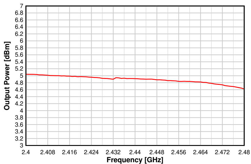
Figure 8-23. Output Power vs. Frequency (BLE 1 Mbps, 2.44 GHz, +5 dBm)
