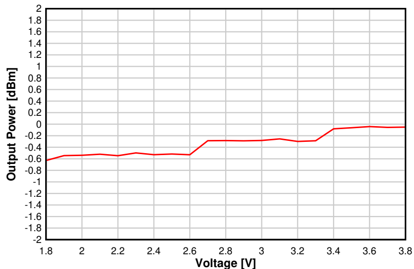
Figure 8-20. Output Power vs. Supply Voltage (VDD5) (BLE 1 Mbps, 2.44 GHz, 0 dBm)
