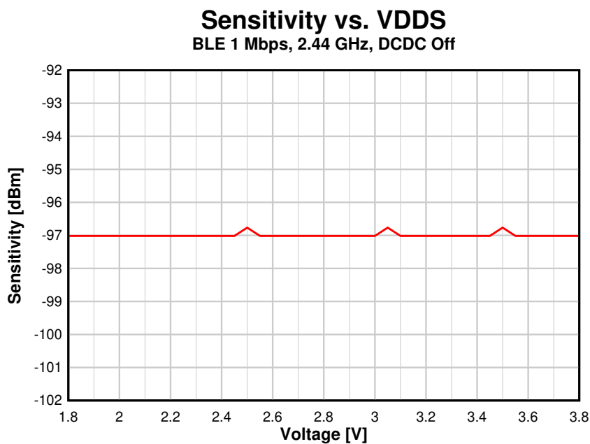
Figure 8-16. Sensitivity vs. Supply Voltage (VDDS) (BLE 1 Mbps, 2.44 GHz, DCDC Off)
