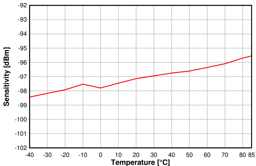
Figure 8-13. Sensitivity vs. Temperature (BLE 1 Mbps, 2.44 GHz)
