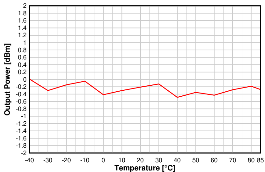
Figure 8-18. Output Power vs. Temperature (BLE 1 Mbps, 2.44 GHz, 0 dBm)
