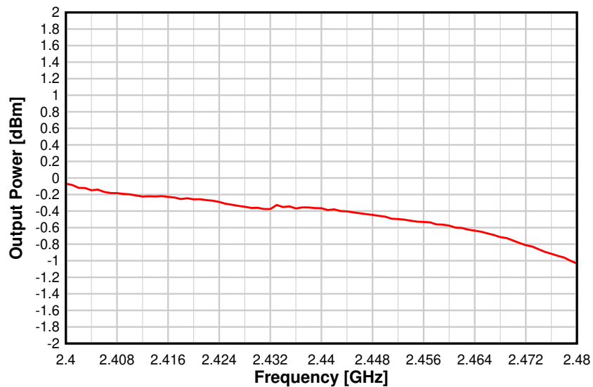
Figure 8-22. Output Power vs. Frequency (BLE 1 Mbps, 2.44 GHz, 0 dBm)
