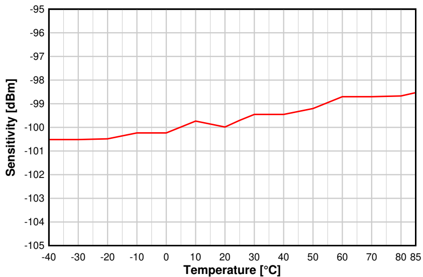
Figure 8-14. Sensitivity vs. Temperature IEEE 802.15.4 (OQPSK DSSS1:8, 250 kbps)
