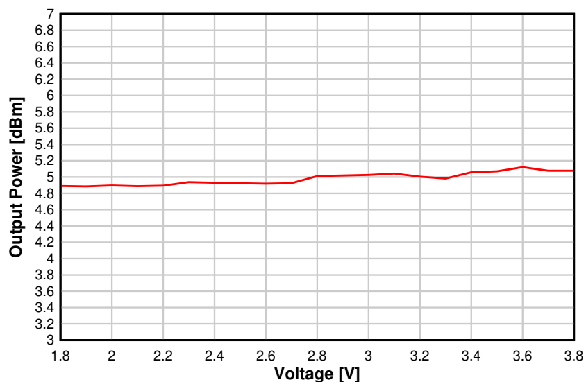
Figure 8-21. Output Power vs. Supply Voltage (VDD5) (BLE 1 Mbps, 2.44 GHz, +5 dBm)
