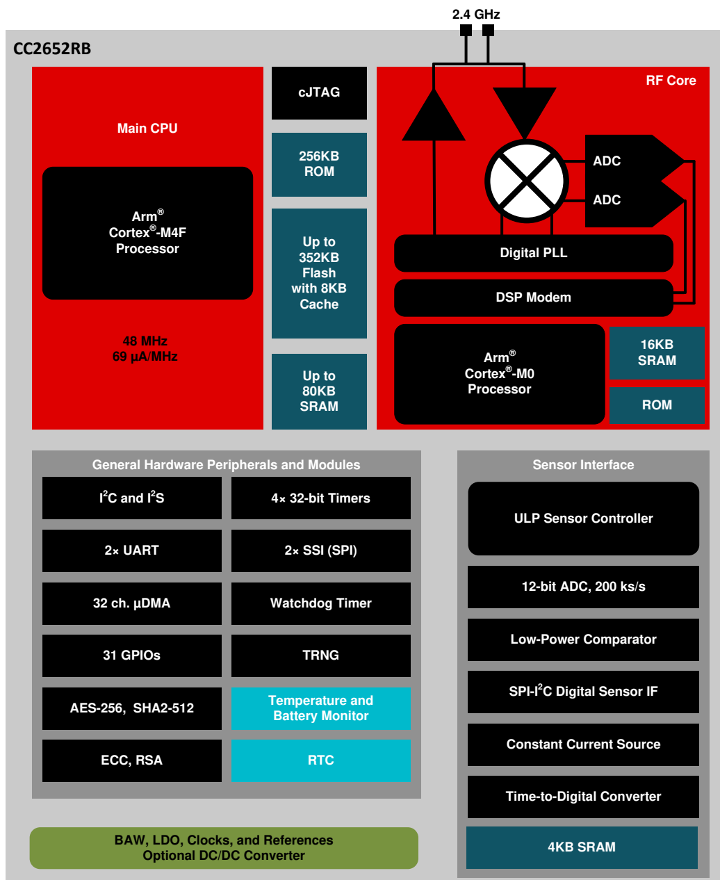
Figure 4-1. CC2652RB Block Diagram
