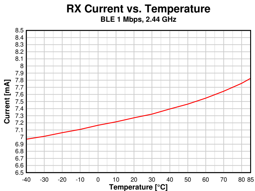
Figure 8-7. RX Current vs. Temperature (BLE 1 Mbps, 2.44 GHz)
