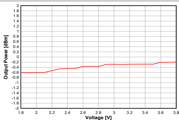
Figure 8-19. Output Power vs. Supply Voltage (VDD) (BLE 1 Mbps, 2.44 GHz, 0 dBm)
