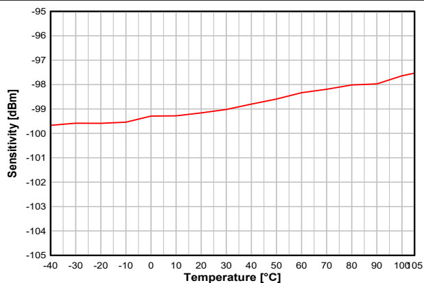
Figure 8-13. Sensitivity vs. Temperature (IEEE 802.15.4-2006, 250 kbps, OQPSK DSSS 1:8, 2.44 GHz)
