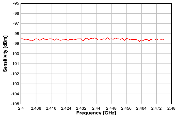
Figure 8-11. Sensitivity vs. Frequency (IEEE 802.15.4-2006, 250 kbps, OQPSK DSSS 1:8, 2.44 GHz)
