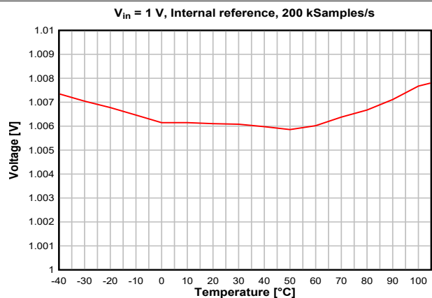
Figure 8-27. ADC Accuracy vs. Temperature
