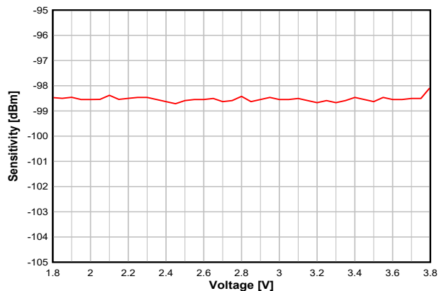
Figure 8-16. Sensitivity vs. Supply Voltage (VDD) (IEEE 802.15.4-2006, 250 kbps, OQPSK DSSS 1:8, 2.44 GHz)
