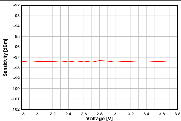
Figure 8-15. Sensitivity vs. Supply Voltage (VDD5) (BLE 1 Mbps, 2.44 GHz, DCDC Off)
