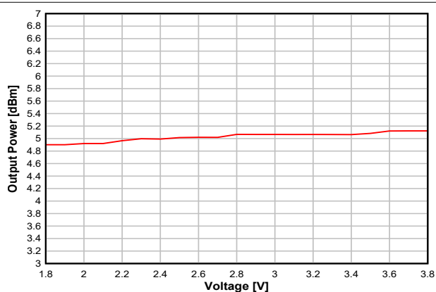
Figure 8-20. Output Power vs. Supply Voltage (VDD) (BLE 1 Mbps, 2.44 GHz, +5 dBm)
