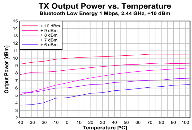
Figure 7-24. Output Power vs. Temperature (2.44 GHz, +10 dBm PA)
