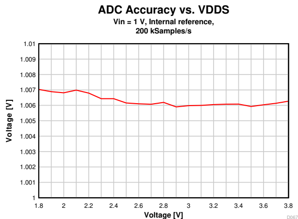
Figure 7-38. ADC Accuracy vs. Supply Voltage (VDD5)
