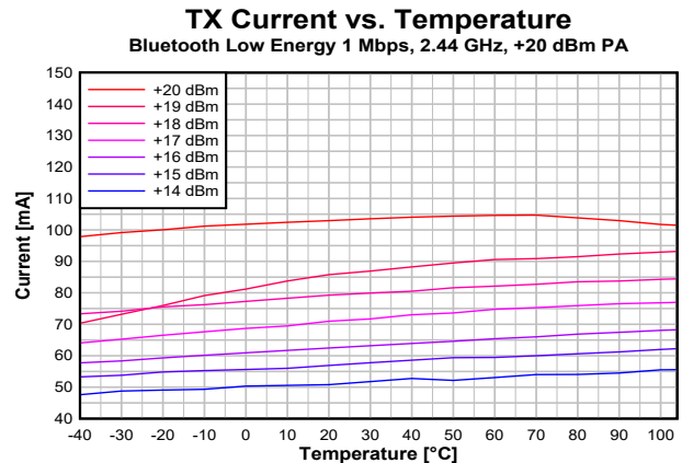
Figure 7-9. TX Current vs. Temperature (Bluetooth Low Energy 1 Mbps, 2.44 GHz, VDD5 = 3.3 V)
