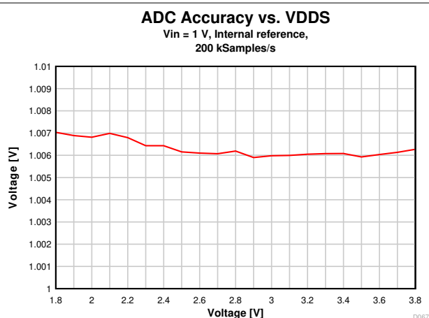
Figure 8-28. ADC Accuracy vs. Supply Voltage (VDD)
