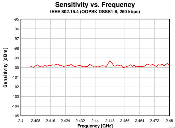
Figure 8-15. Sensitivity vs. Frequency (250 kbps, 2.44 GHz)
