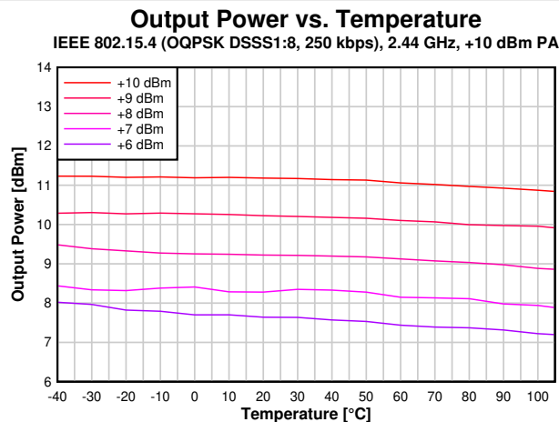
Figure 8-24. Output Power vs. Temperature (2.44 GHz, +10 dBm PA)
