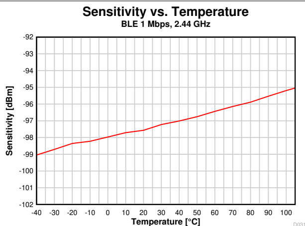
Figure 8-16. Sensitivity vs. Temperature (BLE 1 Mbps, 2.44 GHz)
