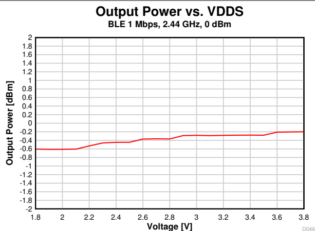
Figure 8-25. Output Power vs. Supply Voltage (VDD5) (BLE 1 Mbps, 2.44 GHz)
