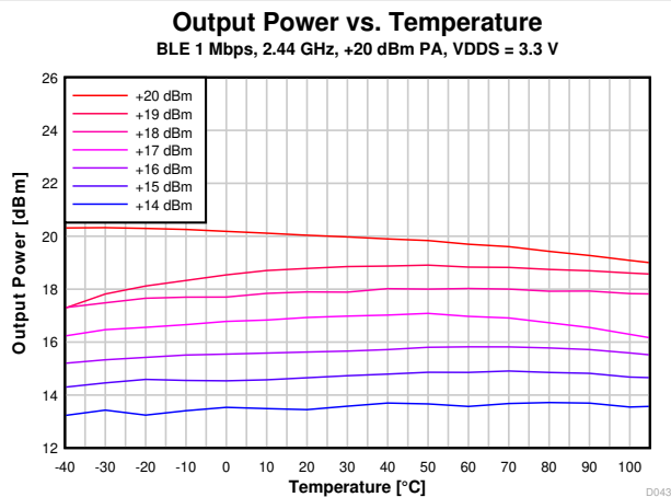
Figure 8-23. Output Power vs. Temperature (BLE 1 Mbps, 2.44 GHz, +20 dBm PA)
