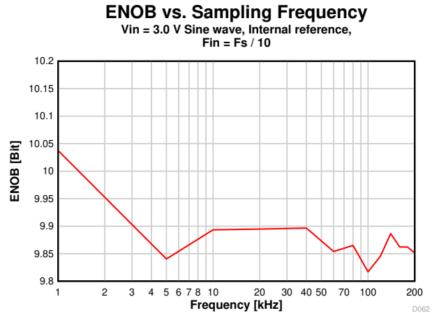
Figure 8-34. ENOB vs. Sampling Frequency
