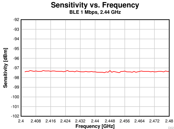
Figure 8-14. Sensitivity vs. Frequency (BLE 1 Mbps, 2.44 GHz)
