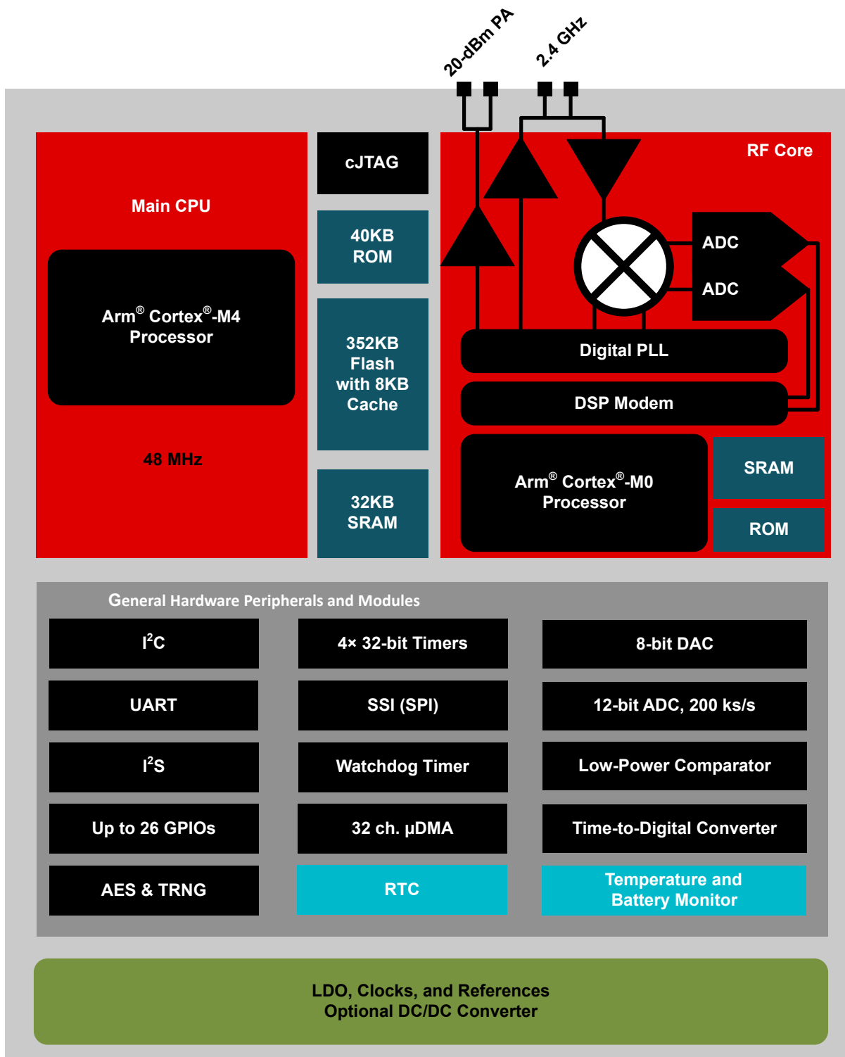
Figure 4-1. CC2651P3 Functional Block Diagram
