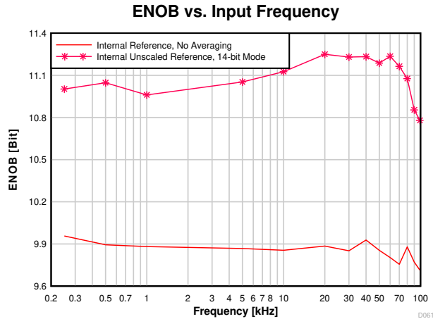
Figure 8-33. ENOB vs. Input Frequency
