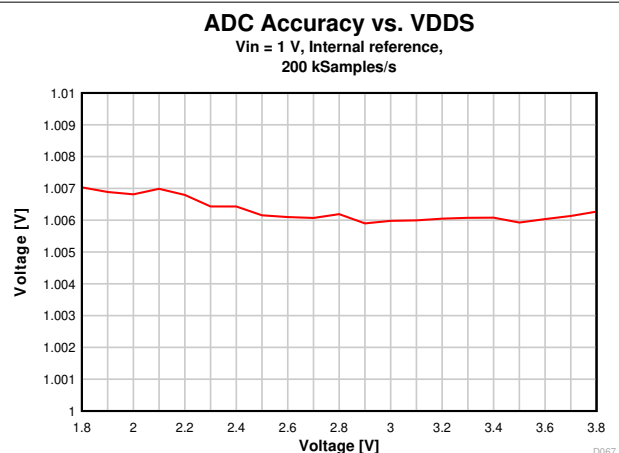
Figure 8-38. ADC Accuracy vs. Supply Voltage (VDD)
