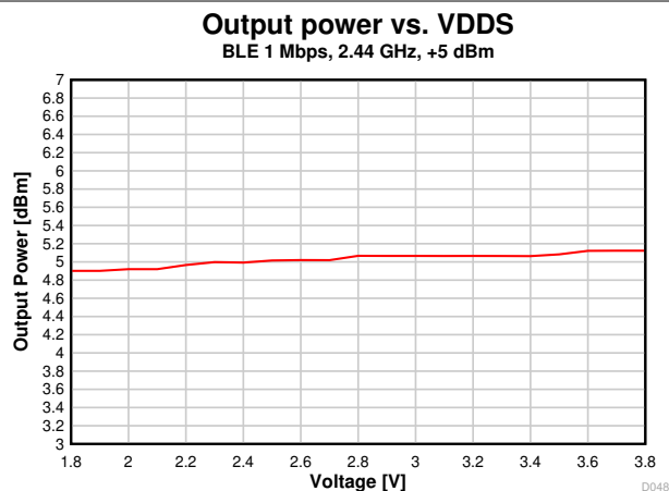
Figure 8-26. Output Power vs. Supply Voltage (VDD5) (BLE 1 Mbps, 2.44 GHz, +5 dBm)
