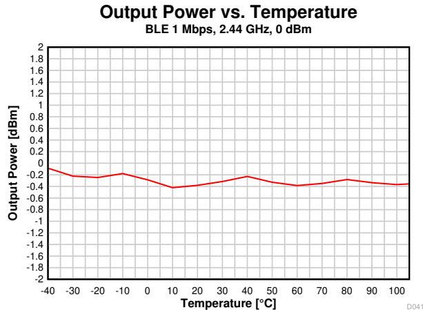
Figure 8-21. Output Power vs. Temperature (BLE 1 Mbps, 2.44 GHz)
