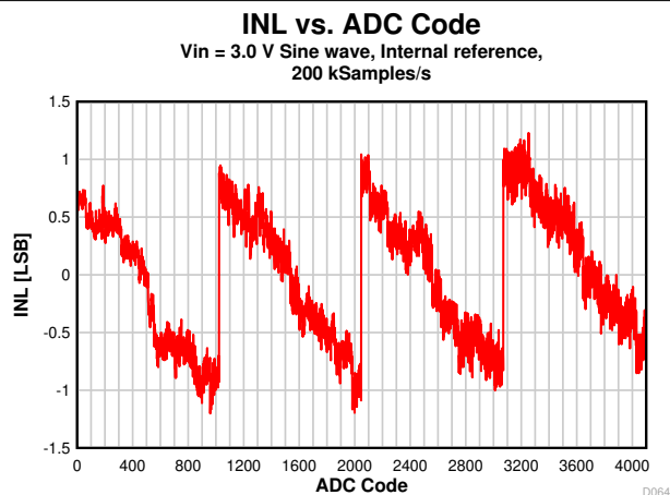
Figure 8-35. INL vs. ADC Code
