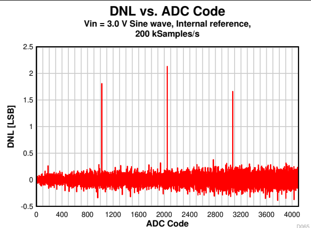
Figure 8-36. DNL vs. ADC Code
