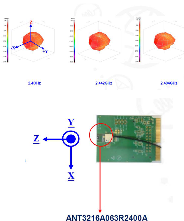
Figure 6-8. Antenna 3-D Radiation Patterns
